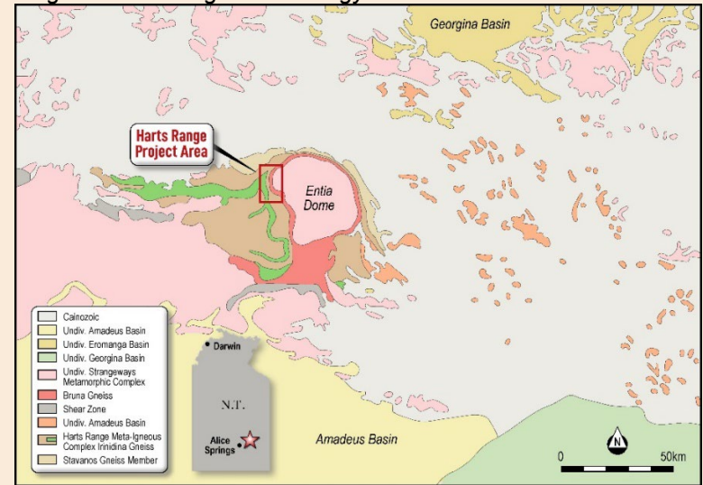
Figure C2-3: Regional Geology
