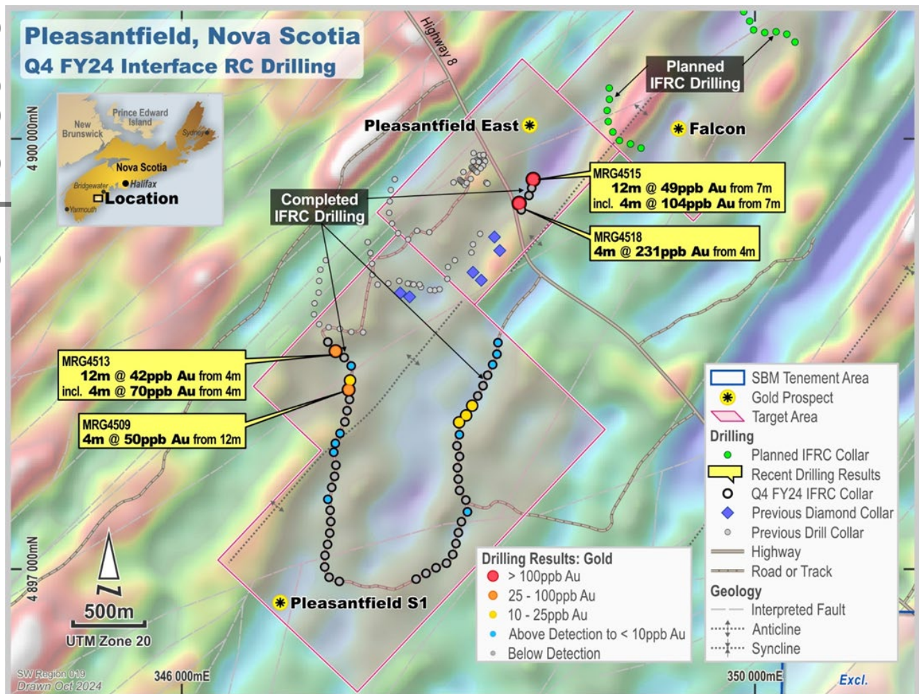
Figure 3. Q1 FY25 Interface RC Drilling Results at Pleasantfield, Nova Scotia, Canada
