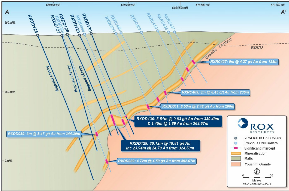
Figure 2: Oblique cross section (A – A' ± 20m) of United North drilling and interpretation looking north.
