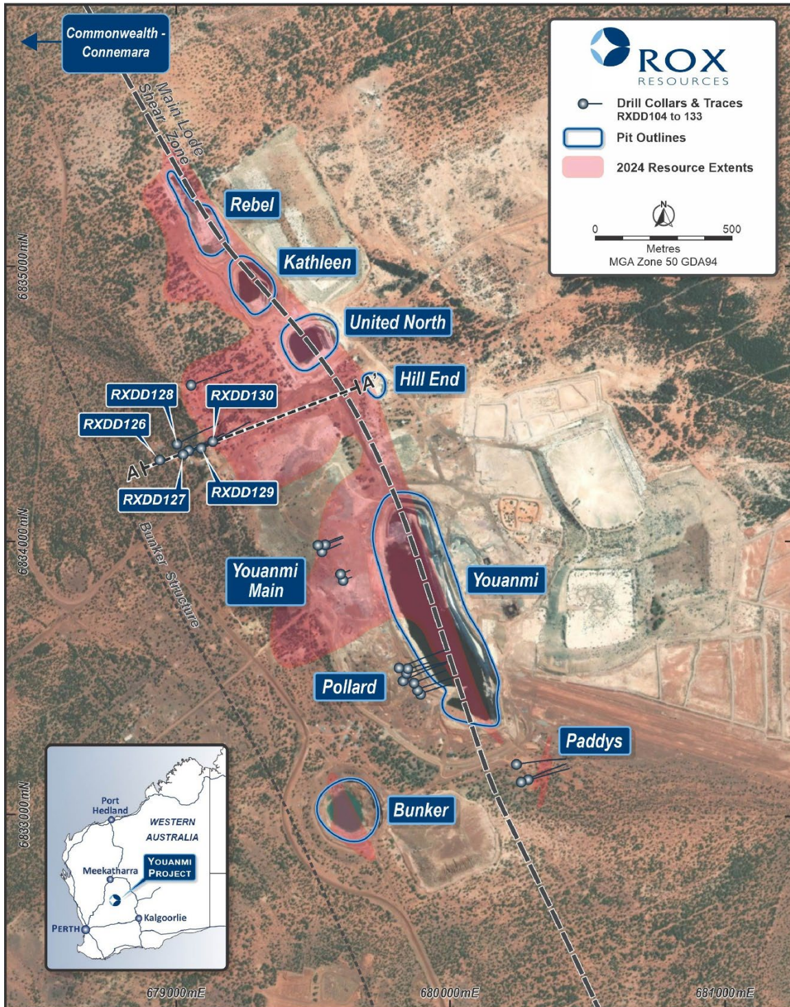
Figure 1: Plan view of the Youanmi Gold Project featuring drill hole collar locations and 2024 Resource outline overlaid on aerial photography.
