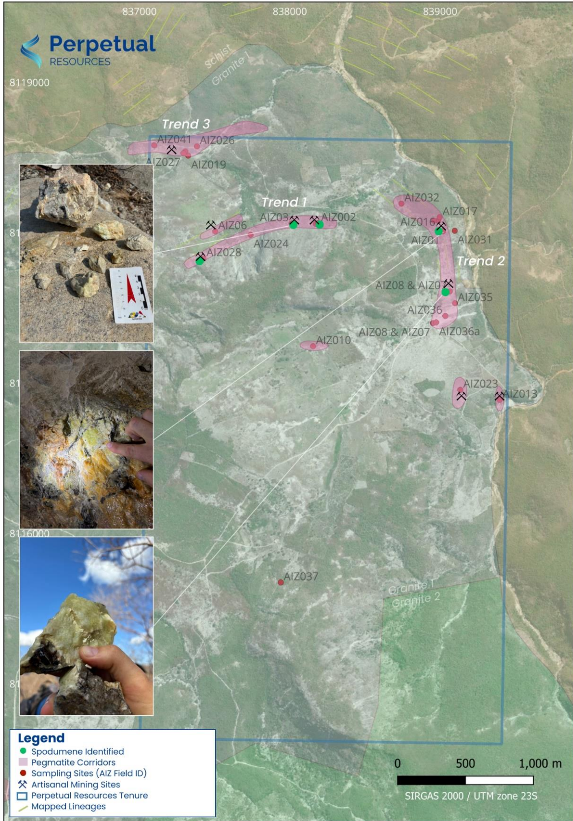
Figure 5: Map showing sampling locations, identified spodumene occurrences, artisanal workings, and pegmatite trends, with an inset photo from field sample work at the Isabella Project. 5
