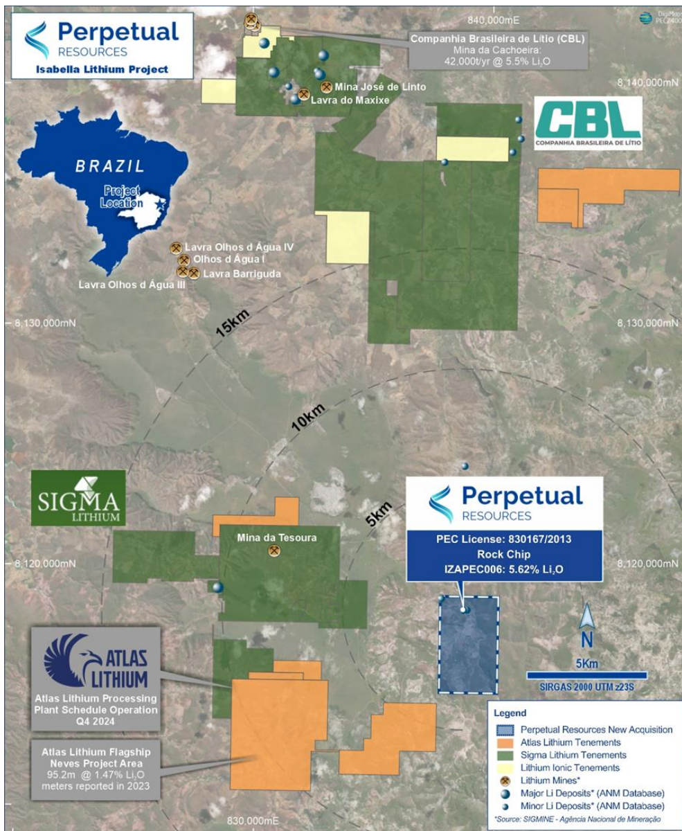
Figure 6 – Regional map of Isabella Project area adjacent to Atlas Lithium and Sigma 678 .
