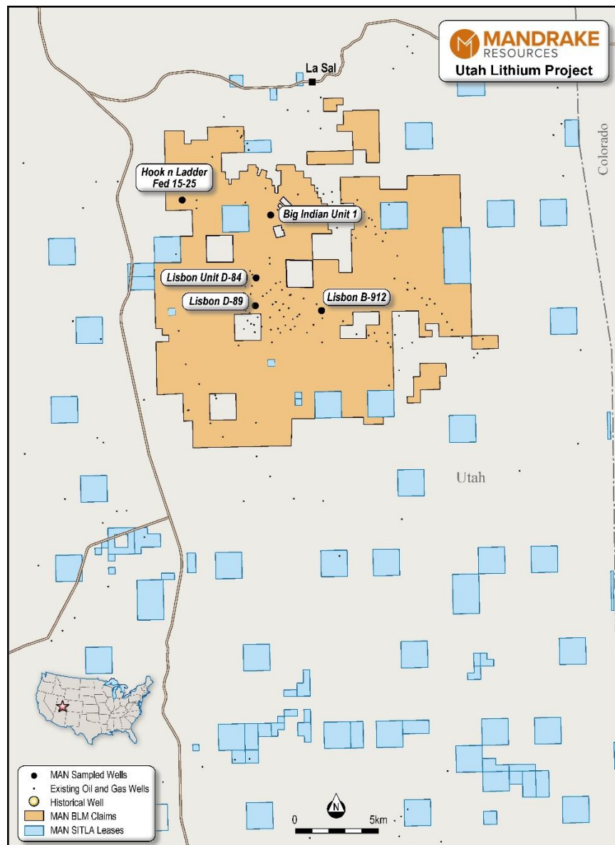
Figure 3. Wells sampled by Mandrake together with existing oil and gas wells used to generate the Mineral Resource Estimate
