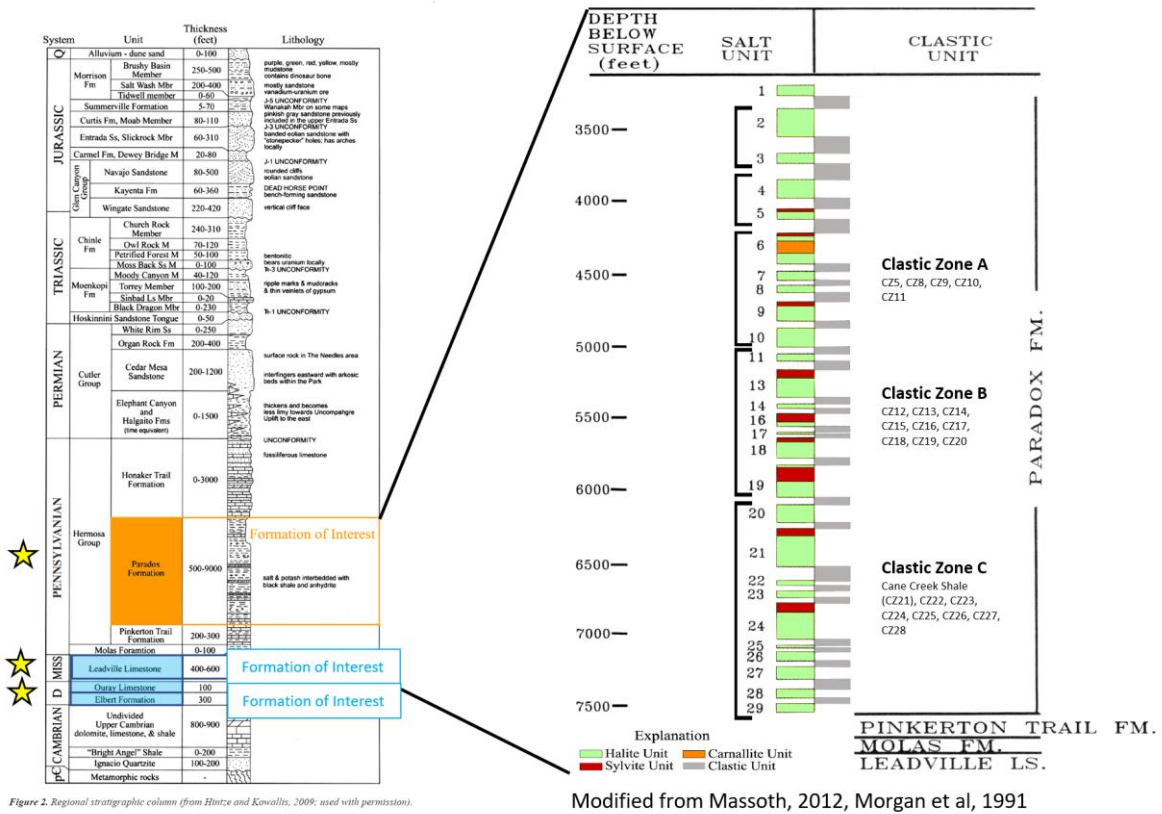
Figure 2. Regional stratigraphic column (from Hintze and Kowallis, 2009; used with permissions).
