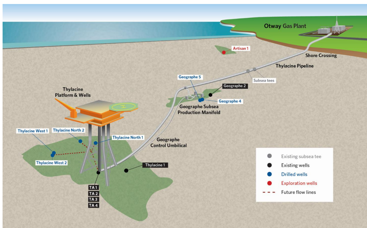
Offshore Otway Basin drilling and development program schematic
