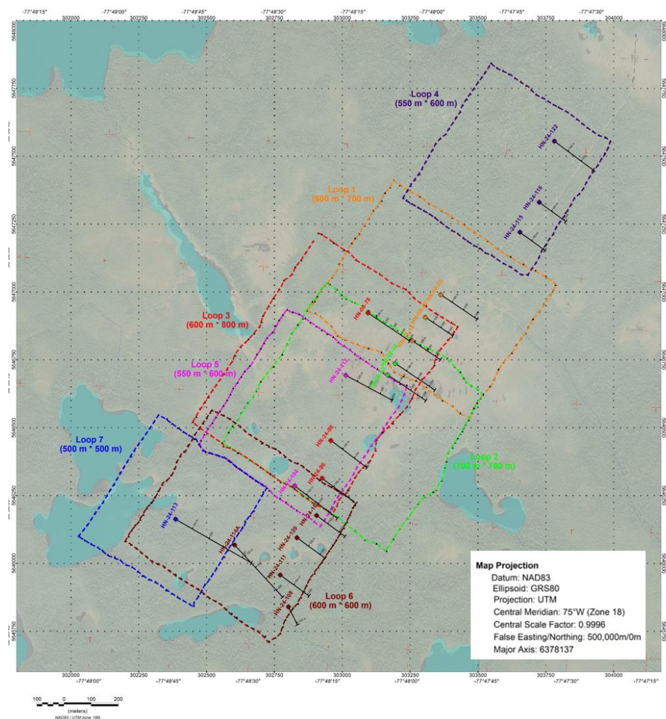
Figure 4: DHEM Loop Locations
