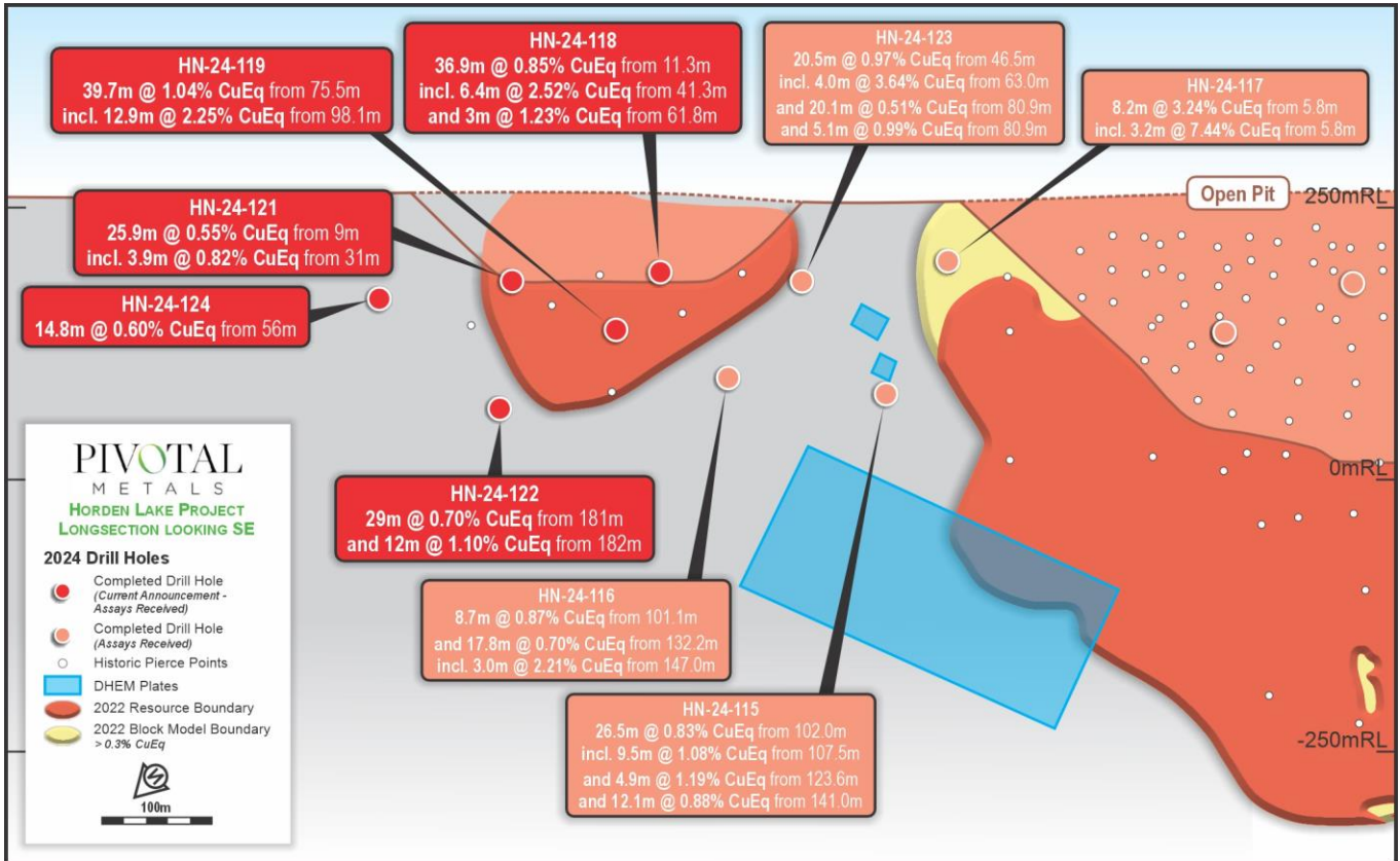
Figure 2: Longitudinal section looking southeast through the Horden Lake deposit, northern zone.
