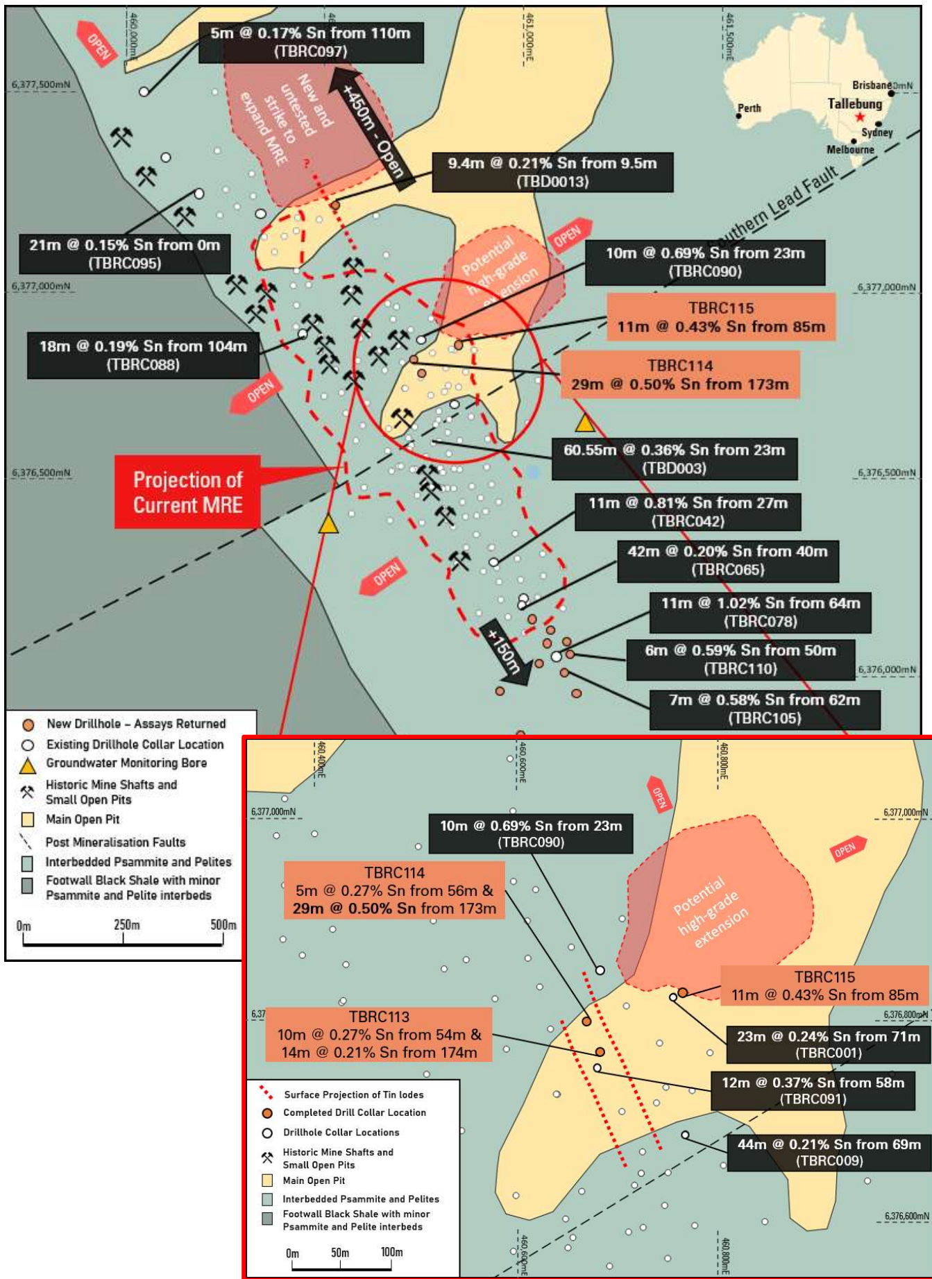
Figure 1: Plan showing the current boundary of the Tallebung MRE with new intercepts shown in orange. Past highlight intercepts are shown in black. Inset shows southern open pit area with new results.
