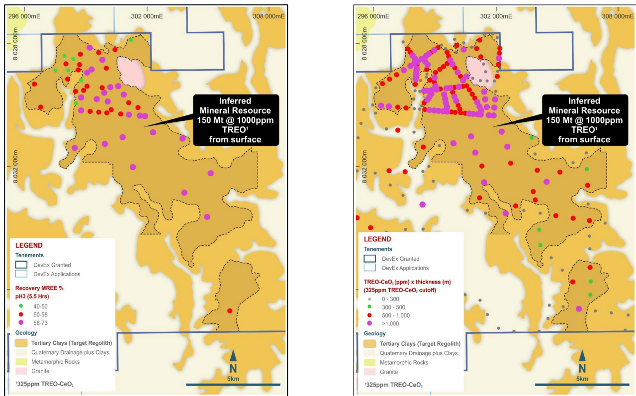
Figure 8. Extent of the Kennedy MRE (black dashed outline) and distribution of MREO mineralisation (right) with MREE recoveries from samples within the resource shown (left).
