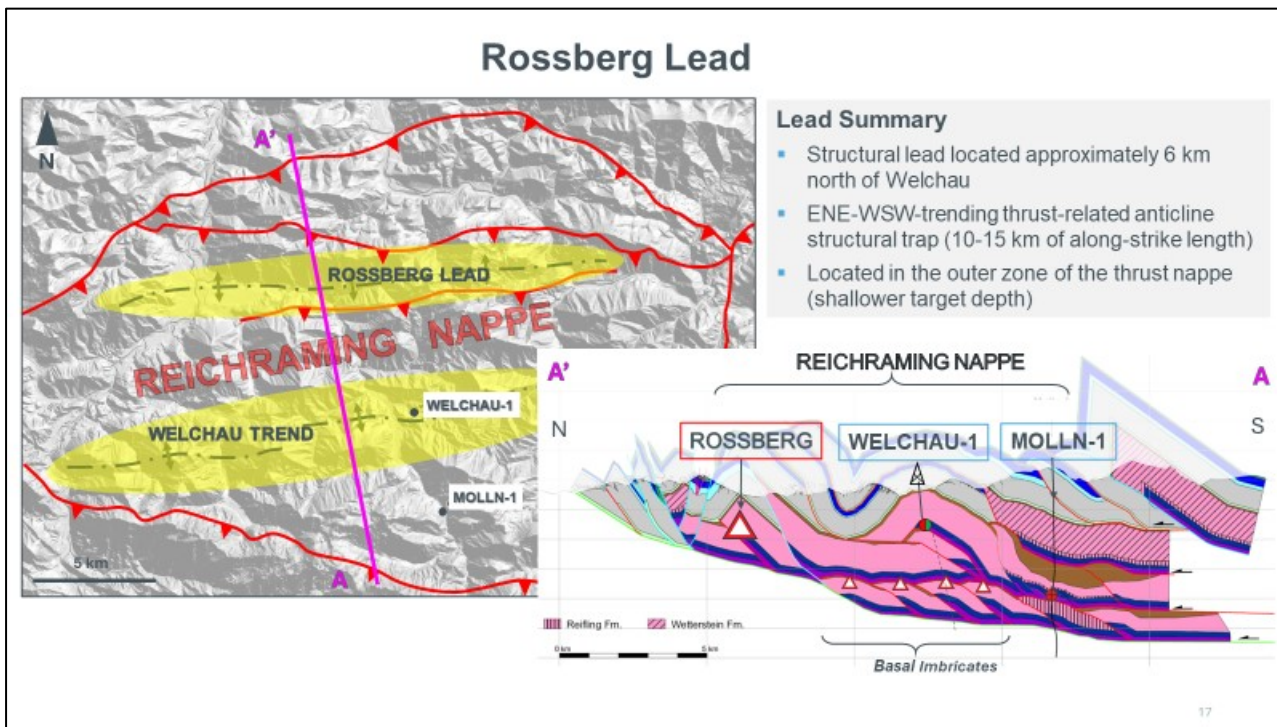
Figure 6: Rossberg lead follow-up exploration to Welchau
