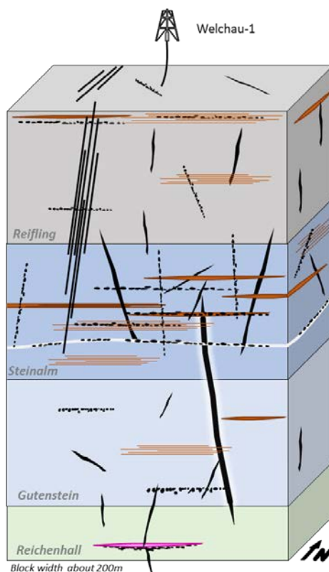
Figure 4: Welchau Carbonates Conceptual Model of an Open Permeable Fracture Network and other transmissibility events seen in the well such as reactivated beddings
