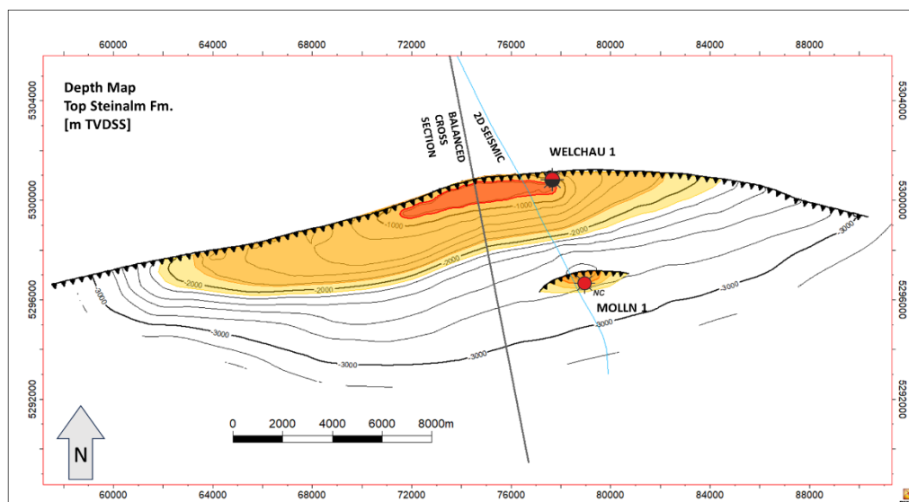
Figure 3: Welchau-1 Top Steinalm Formation post drill map. The 1989 Molln-1 gas discovery is interpreted as a separate accumulation that is not connected to Welchau-1
