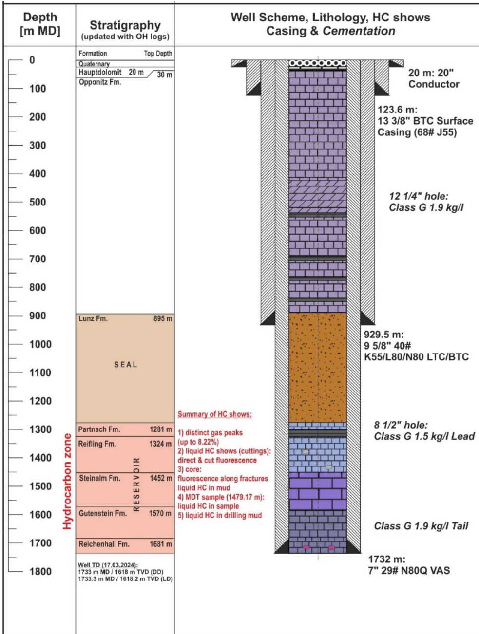
Figure 1: Welchau-1 casing schematic, stratigraphy and hydrocarbon shows encountered while drilling
