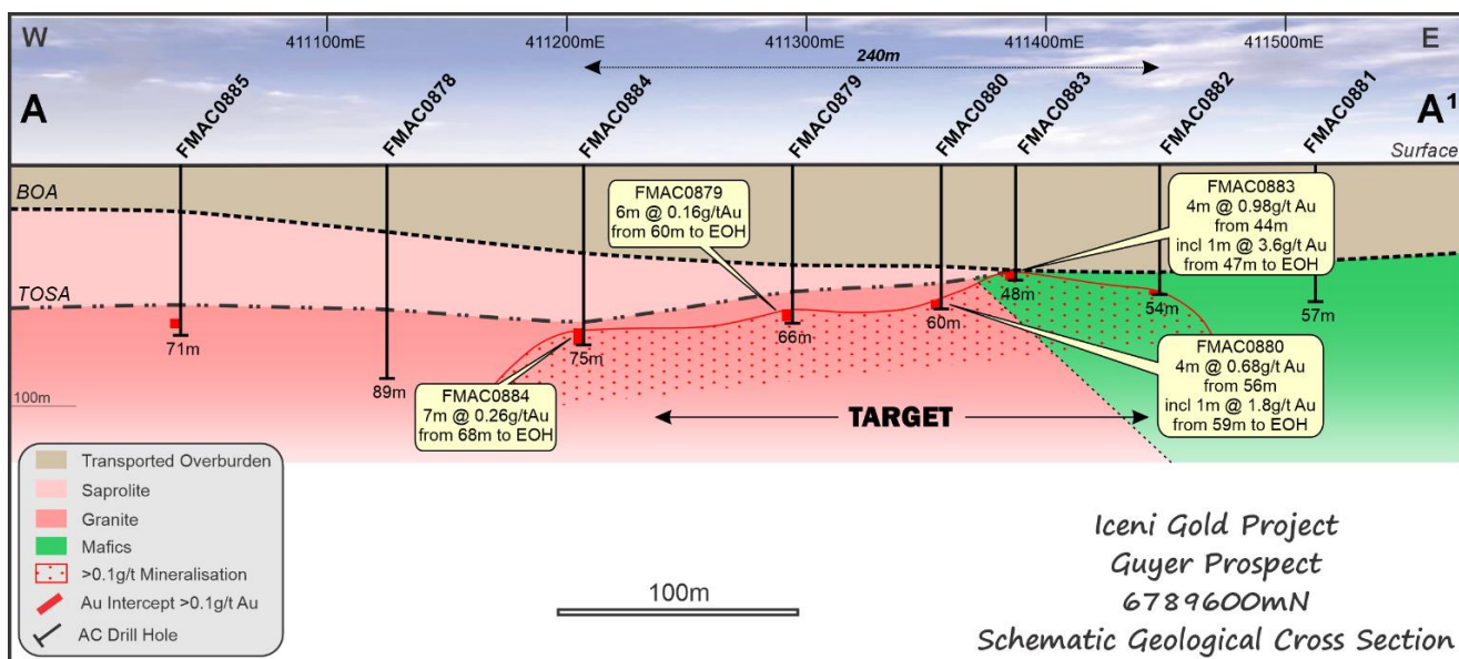
Figure 5: Drillhole cross-section 6789600mN
