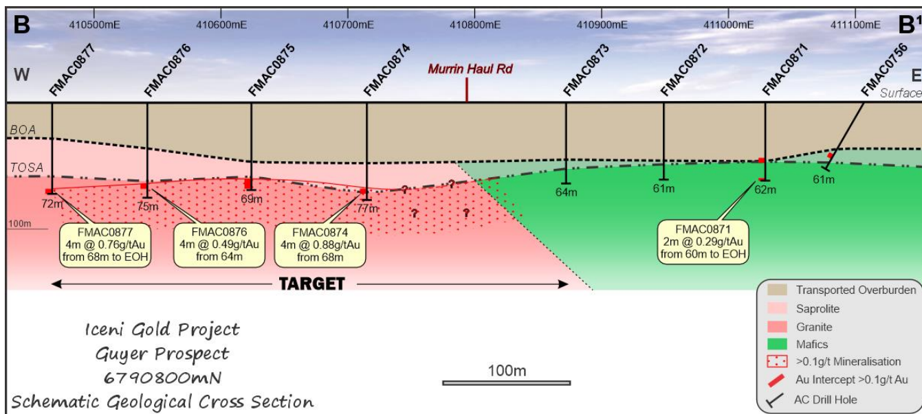
Figure 6: Drillhole cross-section 6790800mN
