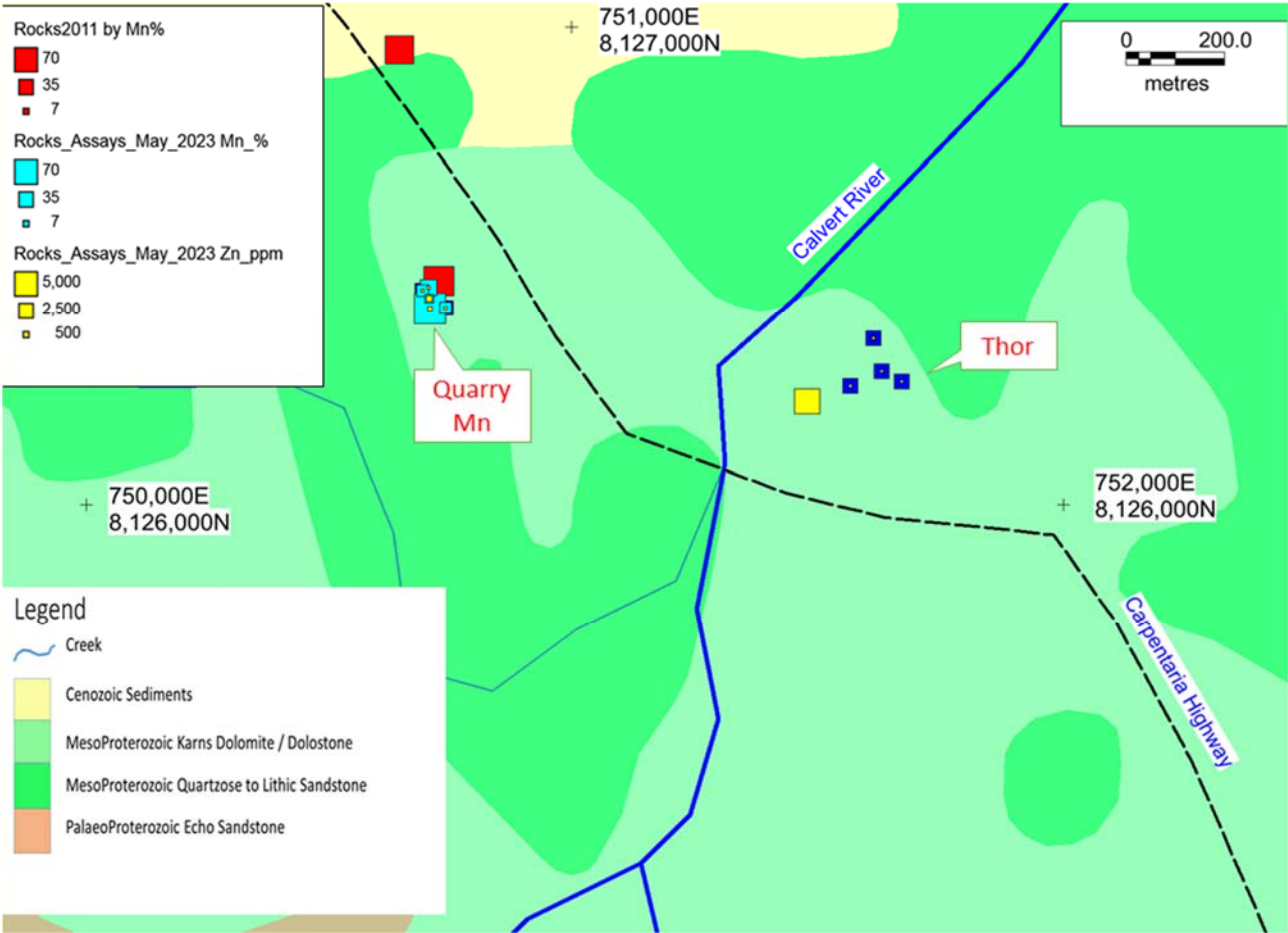
Figure 8 (above) Location of Rock Chip Samples collected on the McArthur River Tenement showing high grade Mn in Light Blue and Moderate Grade Zn in Yellow. Old (2011) Mn samples shown in Red.
