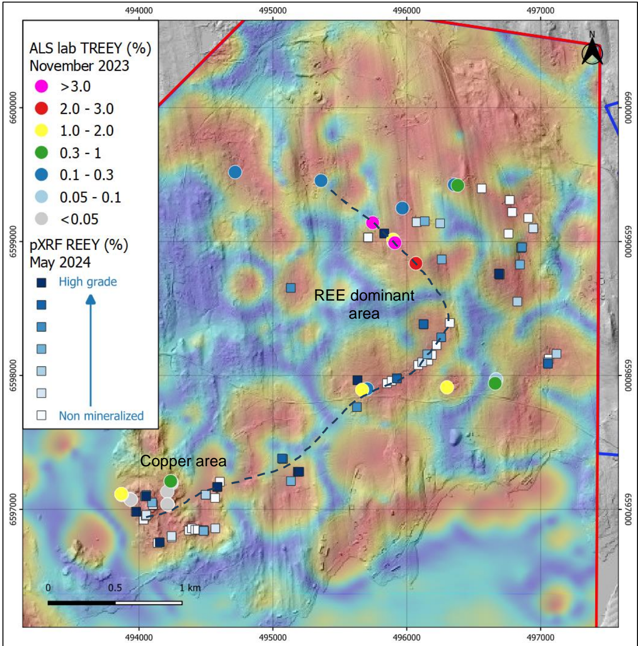
Figure 6: Location of the samples with elevated REE in laboratory assays and pXRF results. The base to the map is the regional magnetic (red magnetic highs, blue lows) with topography superimposed on this. Laboratory assays of REE are shown as circles and pXRF results are shown as squares. The ground magnetic survey is taking place over the area of sampling, to better define the magnetic trends, to assist with drill targeting. The elevated REE trend becomes more copper rich in the south, with the trend extending over approximately 3 km.
