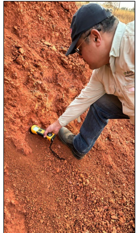
Figure 10: Competent person is assessing the magnetic susceptibility of volcanics on the outcrop
