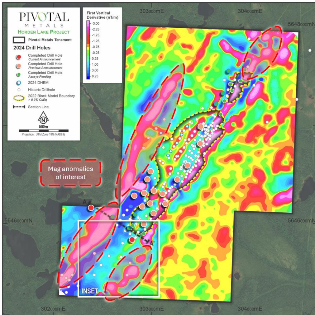
Figure 3: UAV (drone) Magnetic Survey of Horden Lake Project
