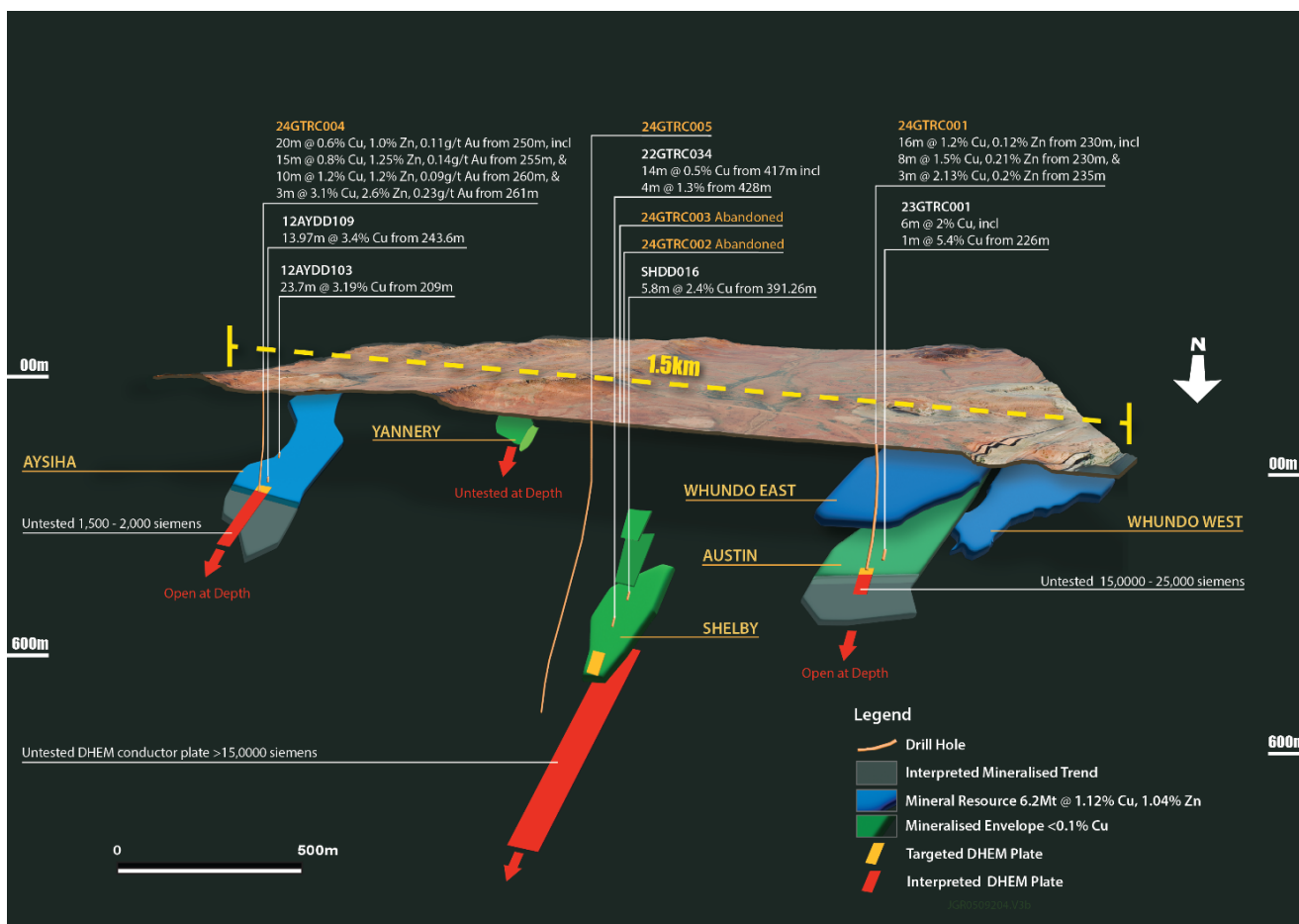
Figure 1: Whundo Cu-Zn VMS Field
