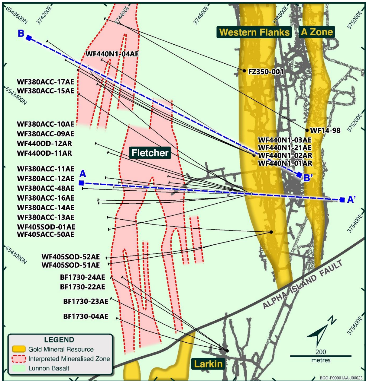
Figure 3 – Southern Stage 1 Exploration Target Area showing existing drilling (refer Figure 1 for location). This area will be subjected to detailed drilling during Q2/Q3 FY25 (Refer to Westgold ASX/TSX Release of 21 August 2024 for full assay results of these drill holes).
