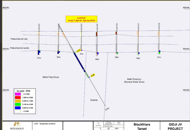
Figure 6. Cross section showing incomplete hole GJRC028 in relation to GJAC627.
