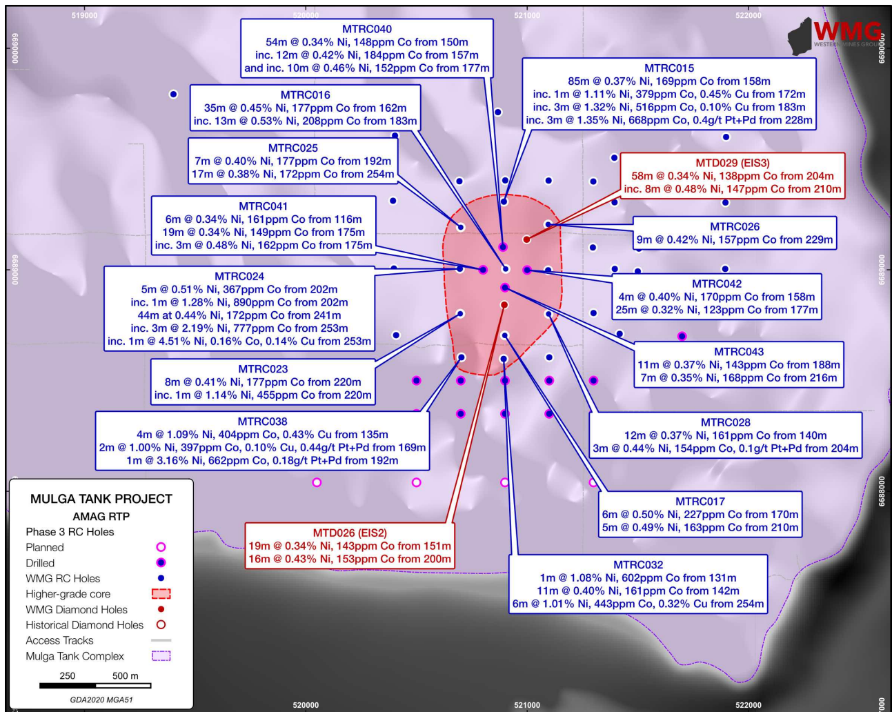
Figure 10: Higher-grade assay results within the core of the Mulga Tank Ultramafic Complex
