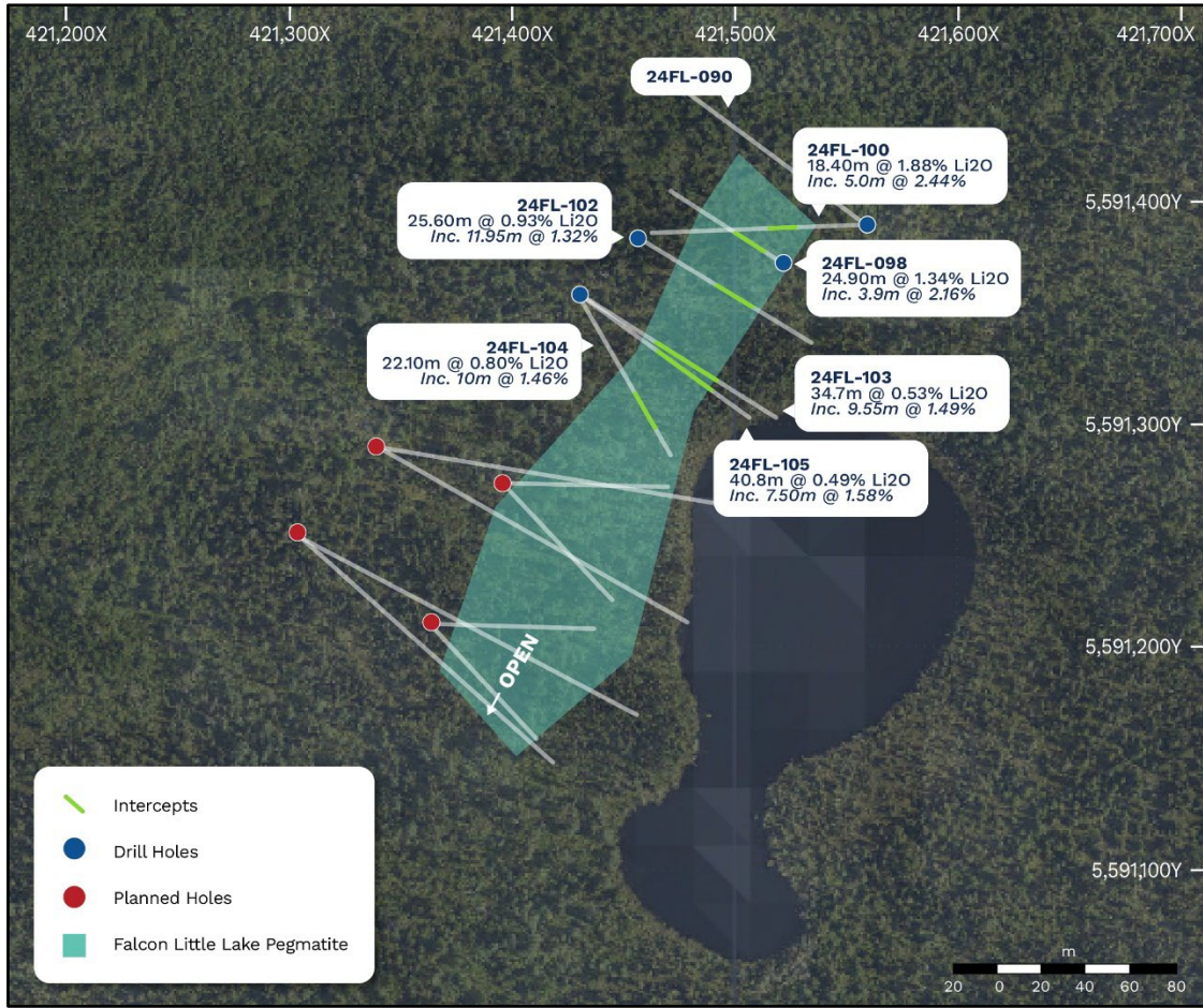
Figure 2 – Falcon Little Lake plan view
