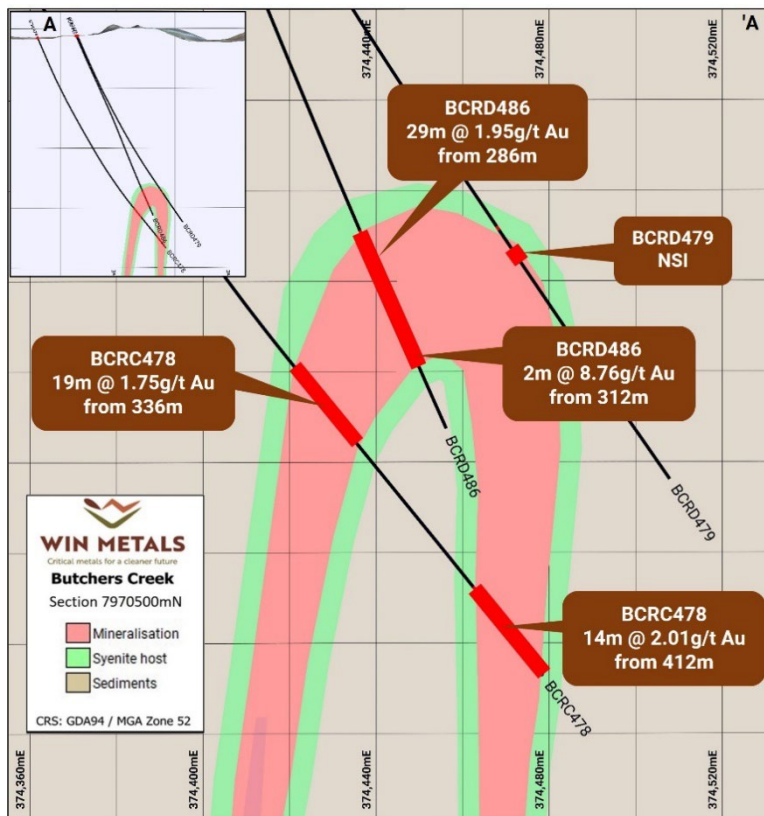
Figure 5 - Schematic section 7970500mN at Butchers Creek illustrating geology and mineralisation
