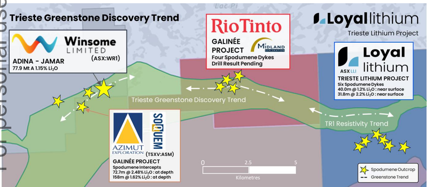
Figure 1: Trieste Greenstone Discovery Trend: Spodumene discoveries across the Trieste Greenstone in relation to Loyal lithium's TRI Resistivity Trend at the Trieste Lithium Project.
