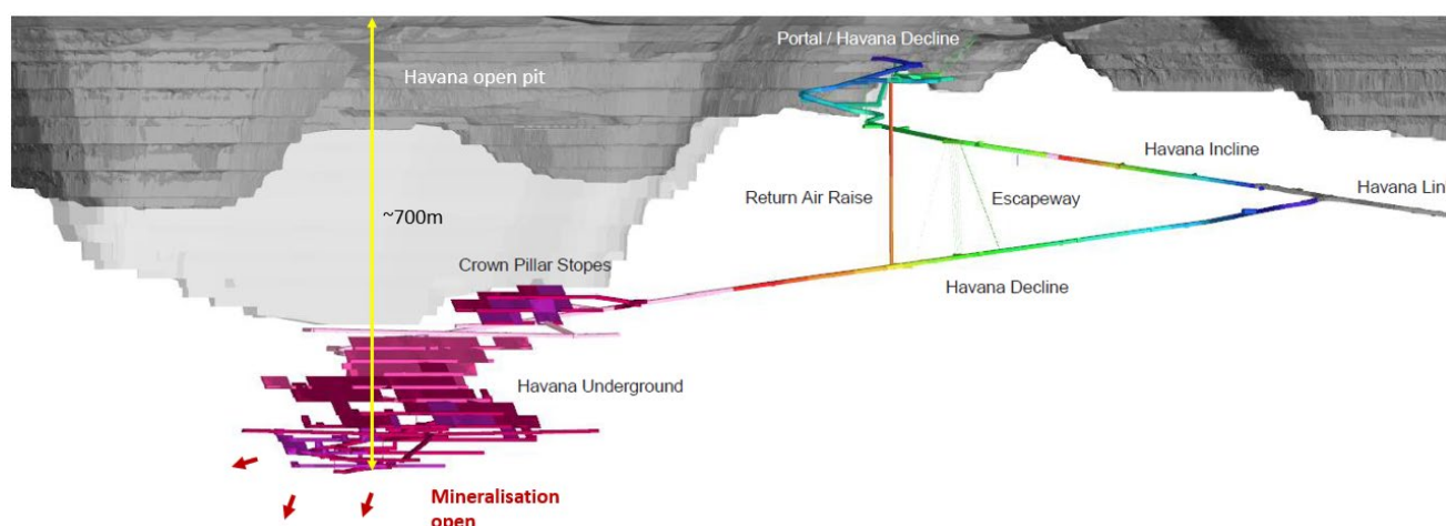
Figure 1: Life of Mine infrastructure design
