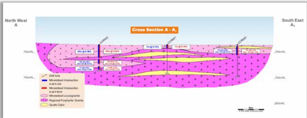
Figure 3: IP Conchas Cross Section A-A1
