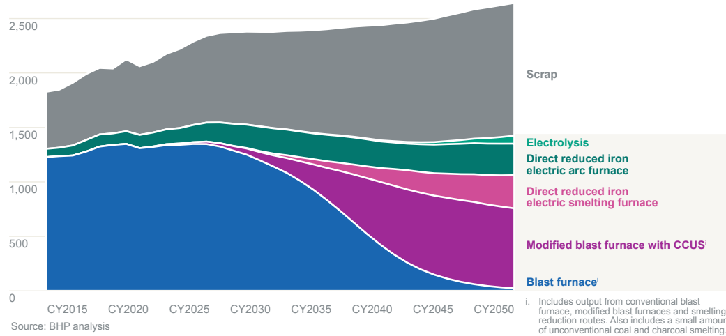
Figure 3.7: Primary iron and scrap use in steelmaking and primary iron making in our 1.5°C scenario Primary iron and scrap use (million tonnes)
