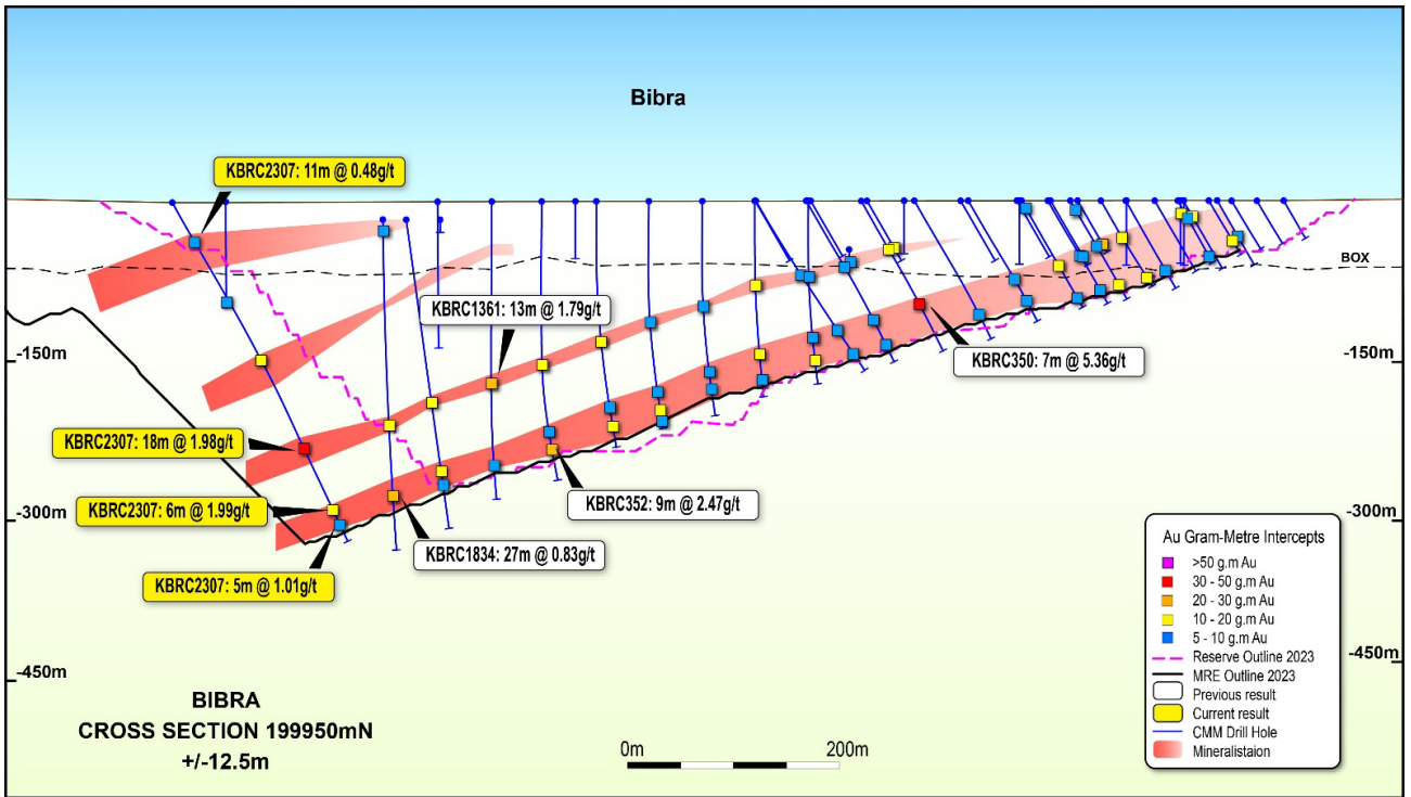
Figure 15. Bibra Section
