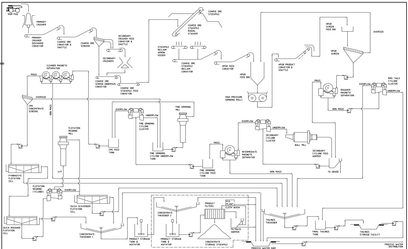
Figure 4: PFS flowsheet (HPGR-Ball mill)
