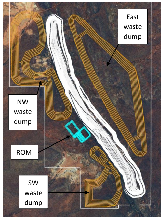
Figure 3: Mining Layout
