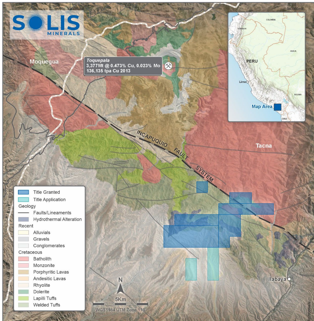
Figure 3: Map of Solis' exploration tenements over regional geology of Cinto Project with the major Incapuquio fault and location of Toquepala mine located 10km to the north west.
