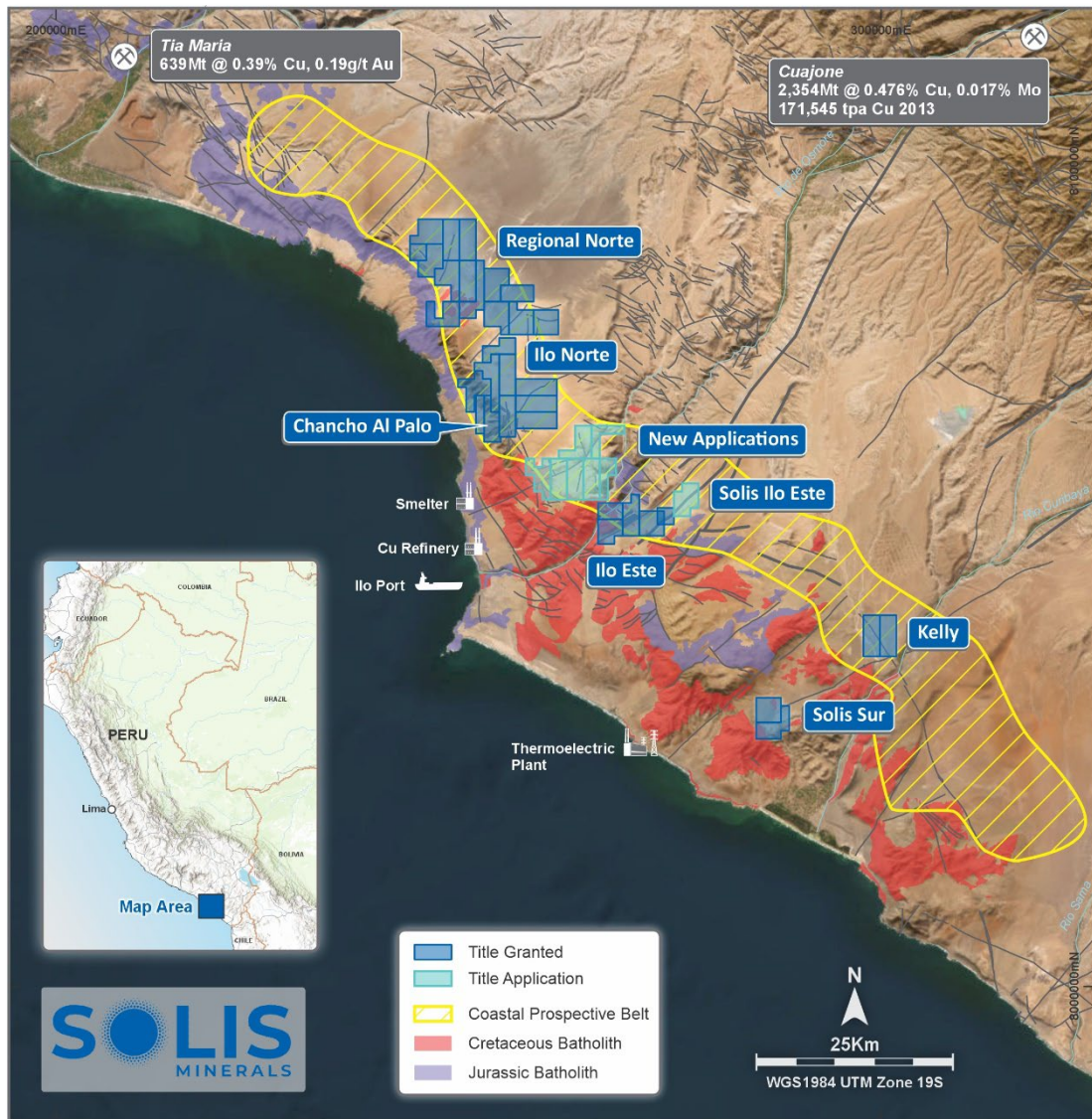
Figure 7: Solis tenements in the prospective coastal belt with existing deposits and regional geology
