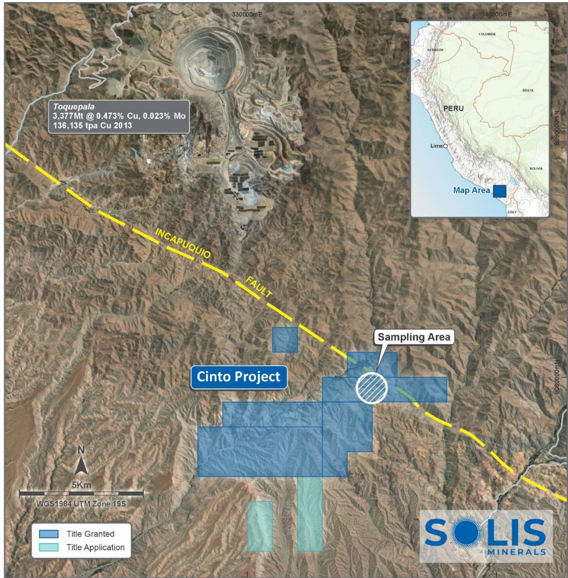
Figure 6: Cinto Project licence areas both under application and granted shown with location of Toquepala mine, owned by Southern Copper Corporation.
