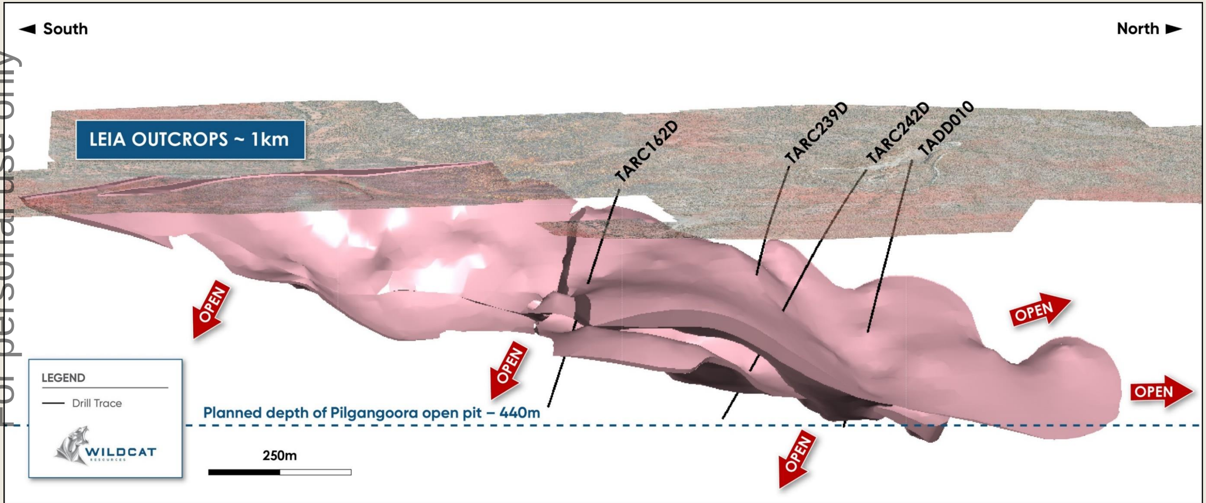
Figure 1 – Isometric view of the evolving geological model for the Leia Pegmatite (pink) with the with the location of recently reported intercepts. Note pegmatite wireframes for the Hutt, Han, Tabbatabba Tantalum, Chewy and Boba prospects are not shown for illustrative clarity. View is looking down towards the west.
