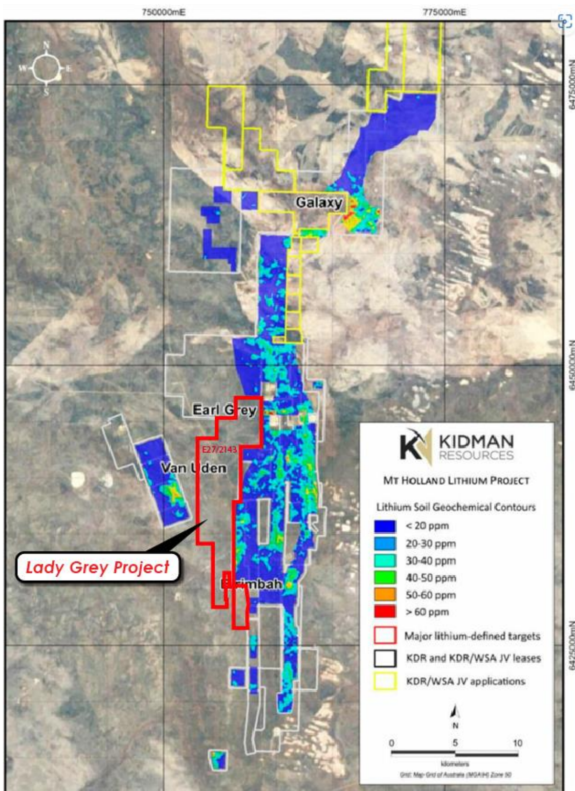
Figure 4: Earl Grey regional soil sampling campaign carried out by Kidman Resource showing >60ppm Lithium anomaly.
