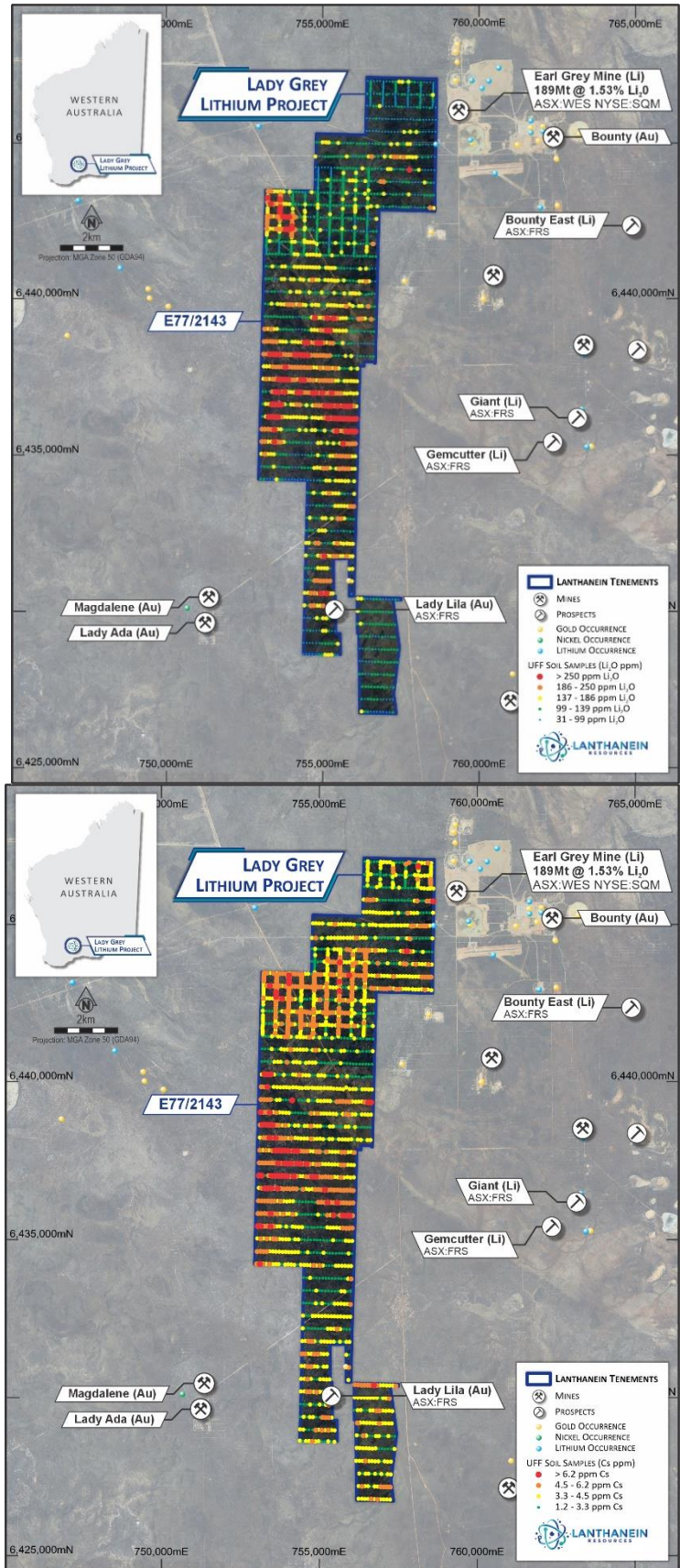
Figure 3: Caesium (Cs) and Lithium (Li 2 O) geochemical results recording strong coincident Cs and Lithium geochemistry supporting potential for presence of LCT-type pegmatites.
