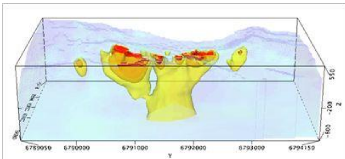
Figure 5: 3D inversion of DIGHEM magnetic data. Isosurfaces: red – 0.15 orange 0.13 yellow 0.11 SI (Fathom Geophysics).
