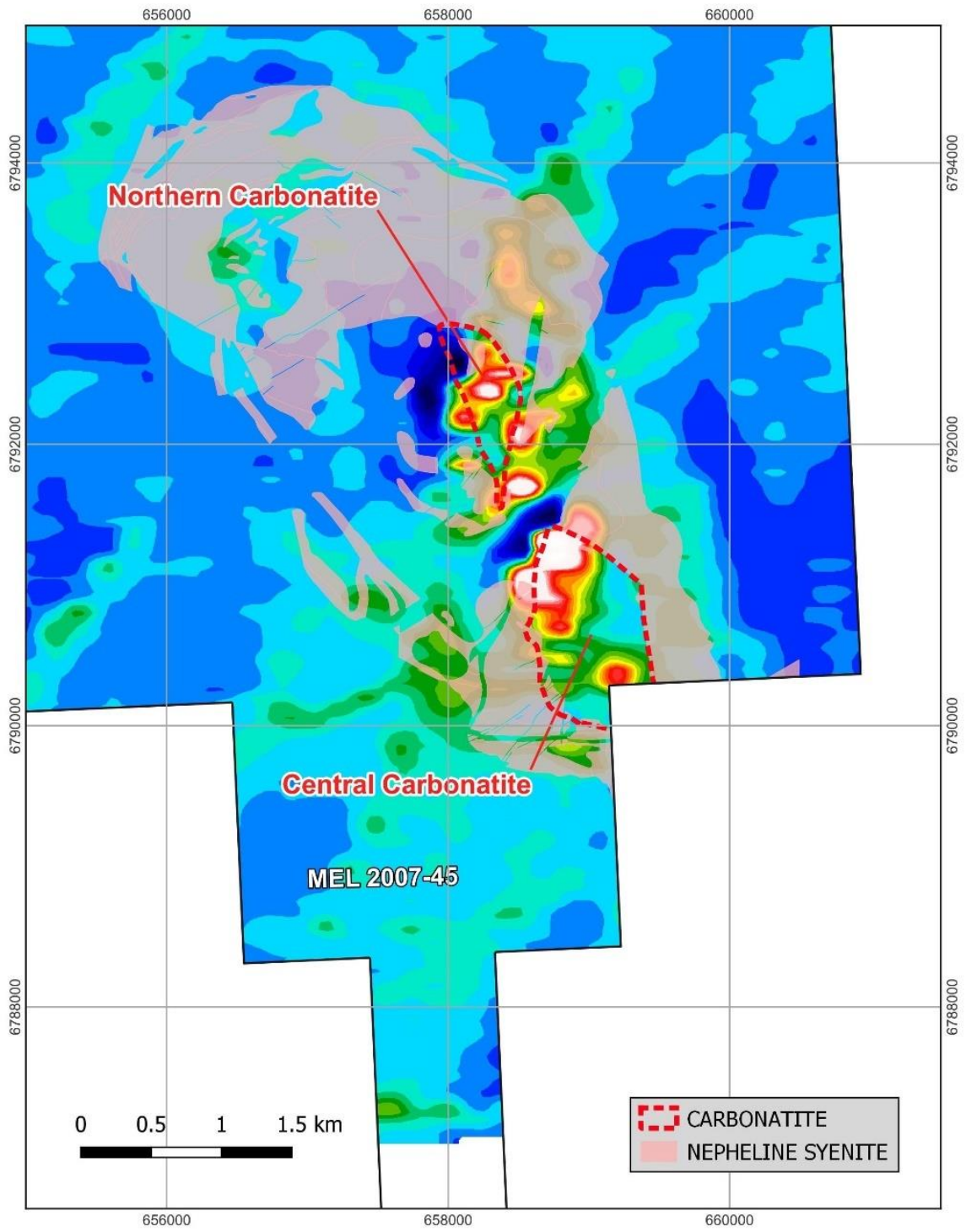
Figure 4: Total magnetic intensity image from DIGHEM survey.
