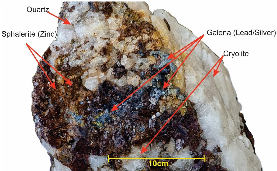
Figure 15: Mineralised waste dump specimen visually estimated to consist of 60% cryolite and quartz; 20% Sphalerite; 10% Galena; 5% Chalcopryrite and 5% Siderite.
