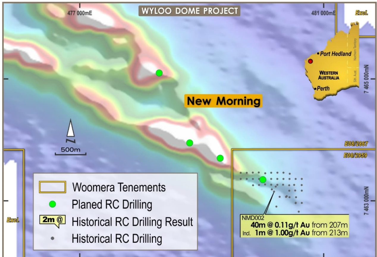
Figure 6: Proposed RC drilling at the New Morning prospect over Channel 48 VTEM imagery
