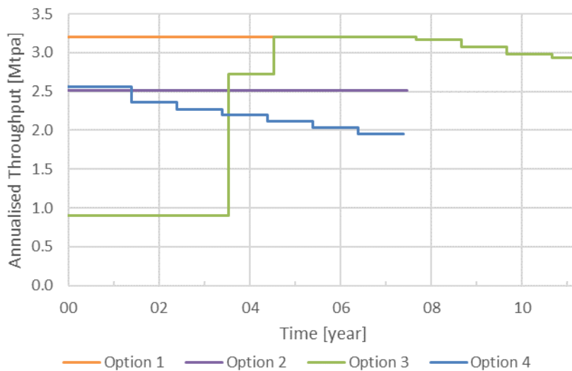
Figure 10-4: TSF K Options Assessment Annualised Throughput at 2.5 m/y Rate of Rise
