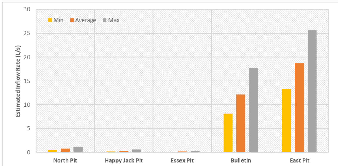
Figure 5-10: Result of groundwater inflow prediction
