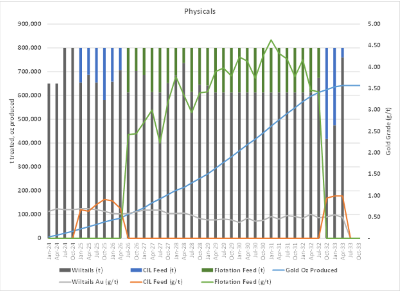
Figure 13a: Production Target Physicals
