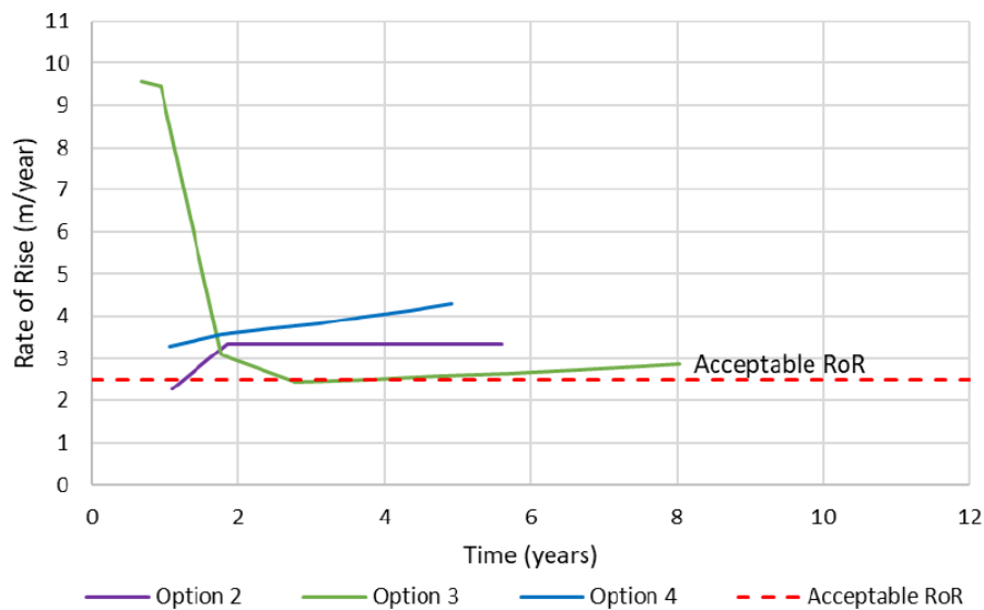
Figure 10-3: TSF K Options Assessment Rate of Rise for 3.2 Mtpa
