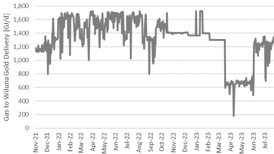
Figure 12-2: Daily Gas Exit at Wiluna Gold Delivery Stream from APA Contract Account
