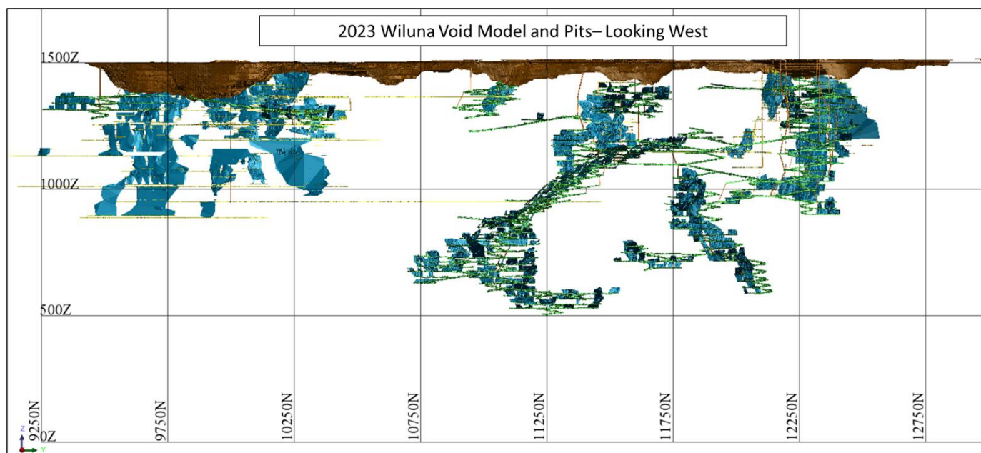
Figure 3-15: Wiluna Void and Pit Depletion Model
