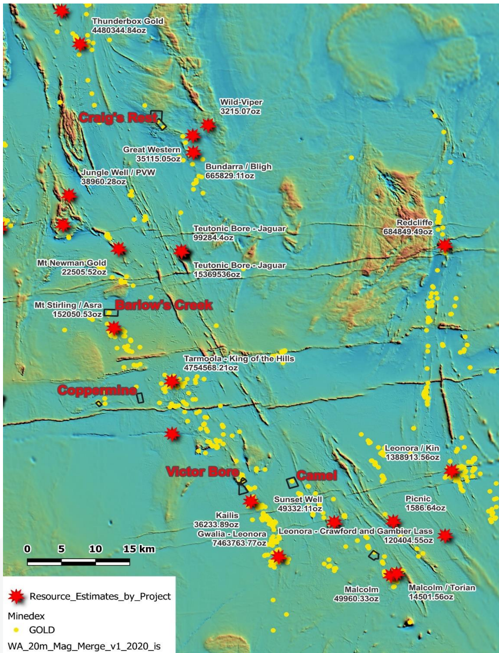
Figure 4 - Regional magnetics showing the IMI goldfields projects, nearby resources and gold discoveries.
