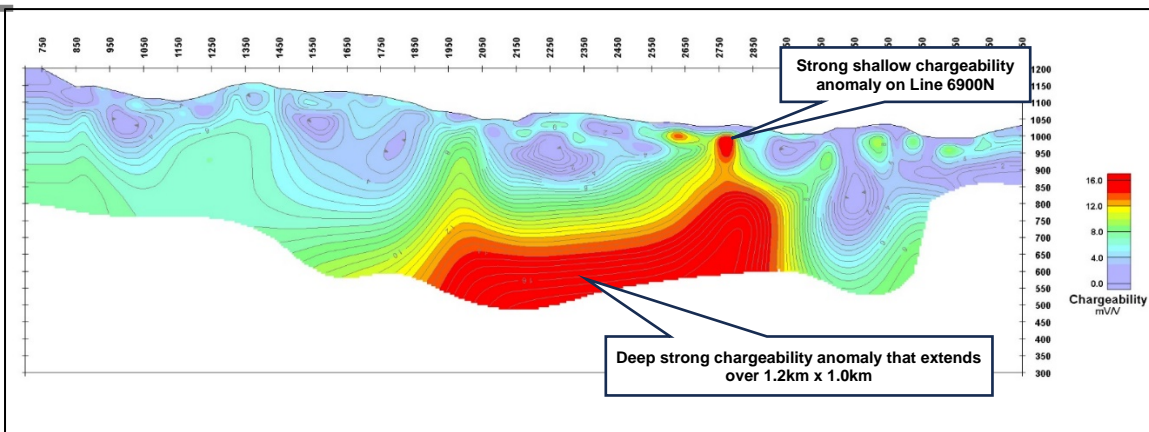
Cross-section showing a depth-inversion of chargeability data from the Discus Copper Prospect (Line 6900N) – illustrating that a small portion of the source of the IP anomaly comes close to surface, but the majority of the source lies “hidden” at depth.
