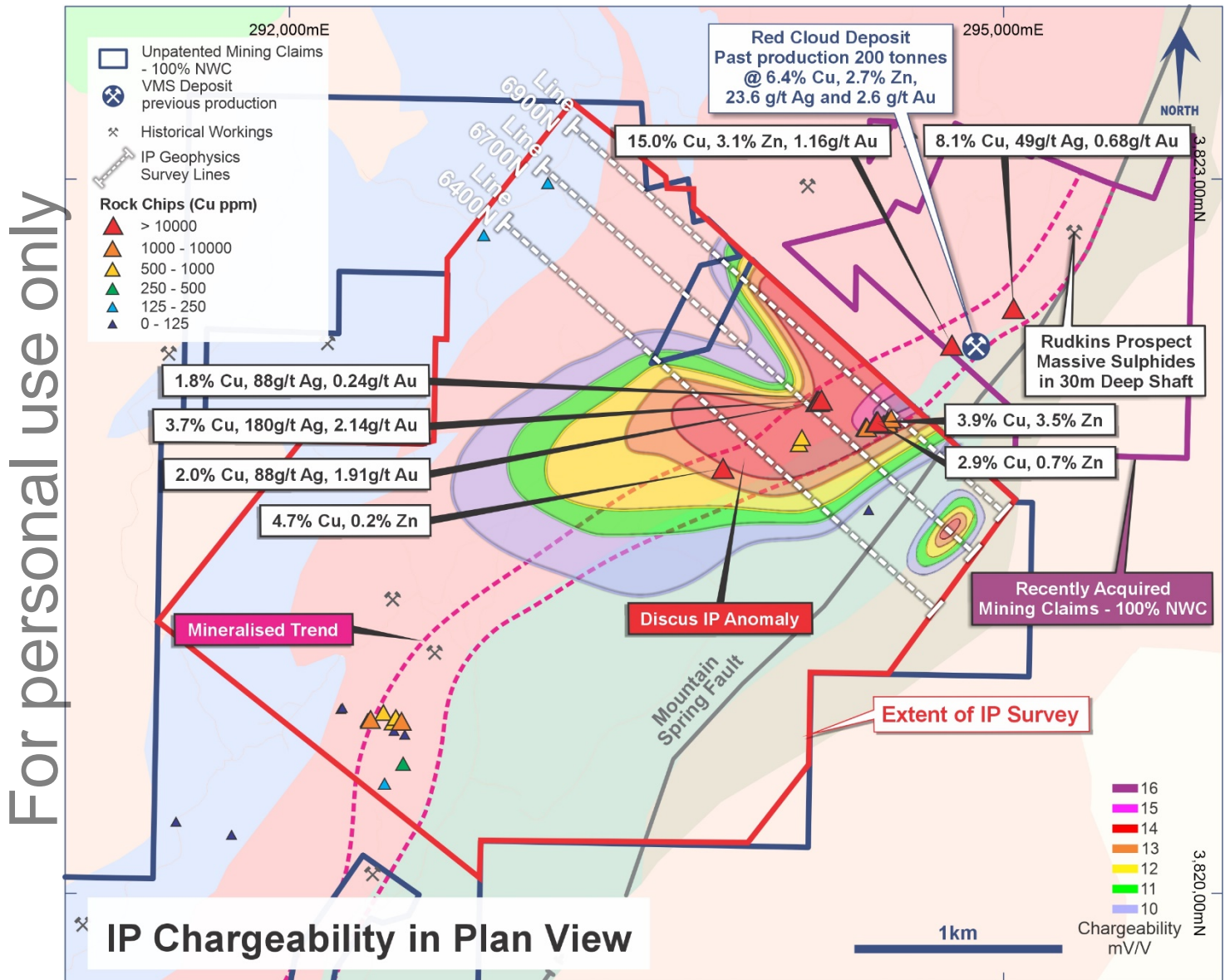
Figure 1. Plan view showing location of rock samples and select assay results, collected recently over the strong Discus IP Anomaly at the Javelin VMS Project. The Discus Prospect is located within a mineralised trend that hosts the recently acquired Red Cloud VMS Deposit as well as massive sulphides at the Rudkins Prospect. Contours show chargeability at the 650m RL (approximately 350-400m below surface) superimposed upon mapped geology.
