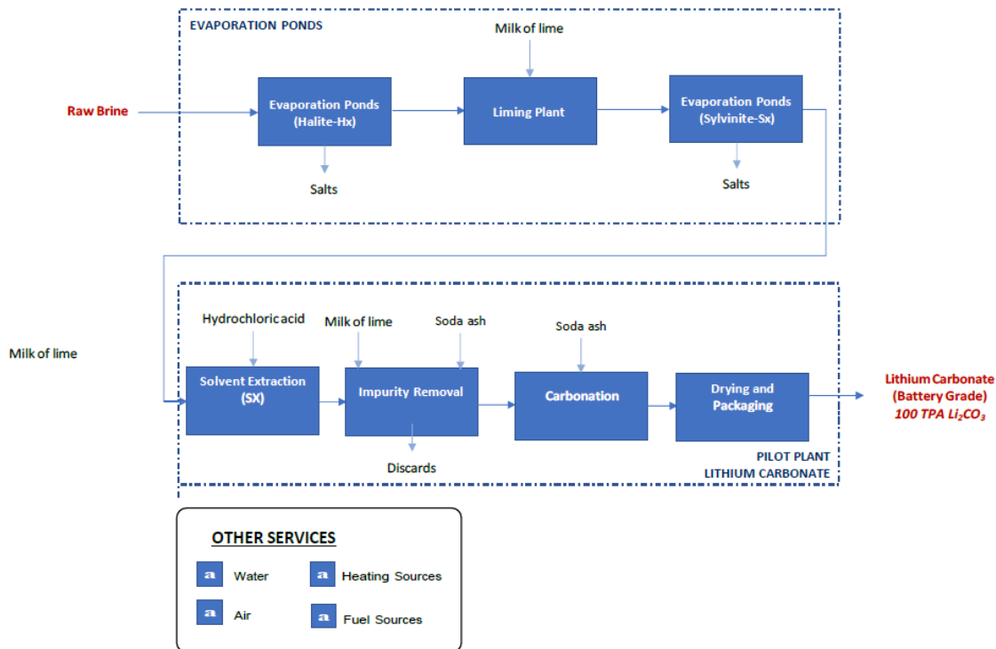
Figure 2 – Block diagram of the main stages of the Evaporation Ponds and Lithium Carbonate Plant
