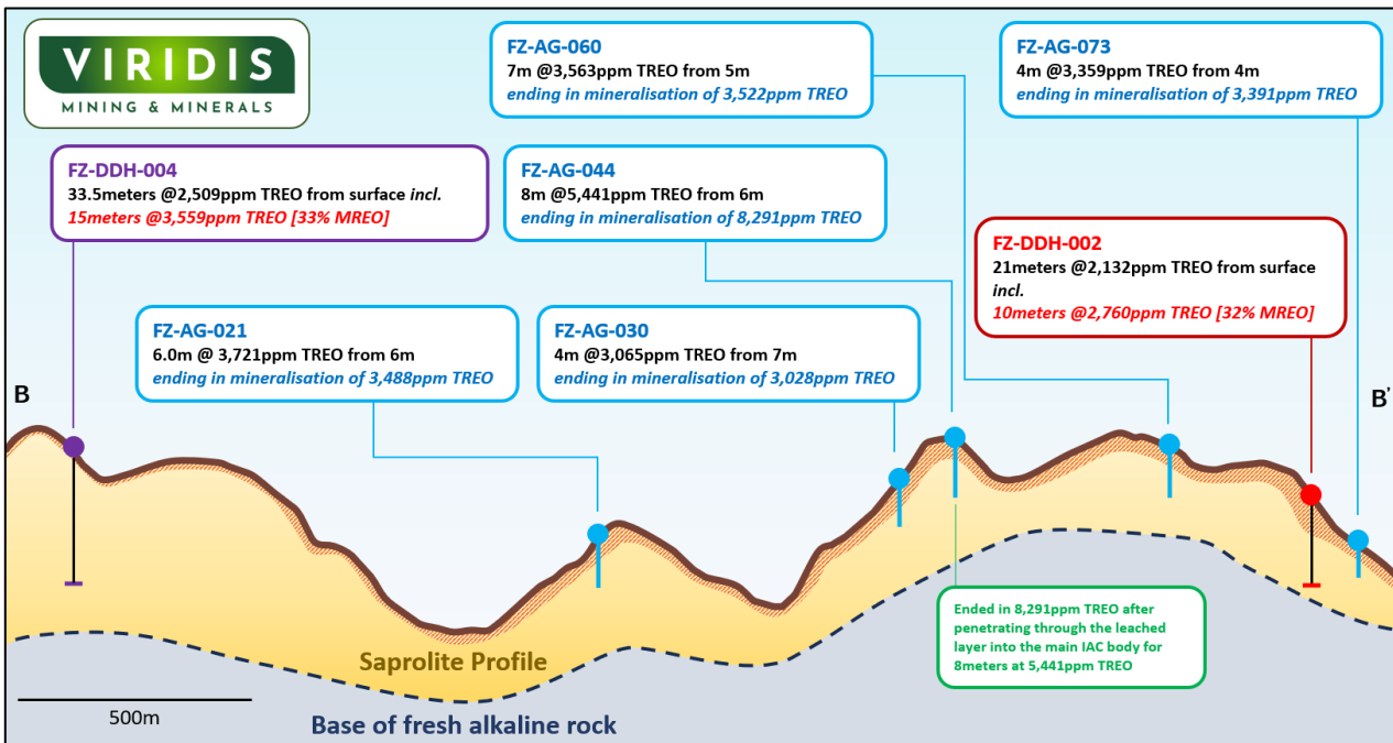
Figure 3: Geological interpretation of cross section BB' going across Fazenda as shown in Figure 1.
