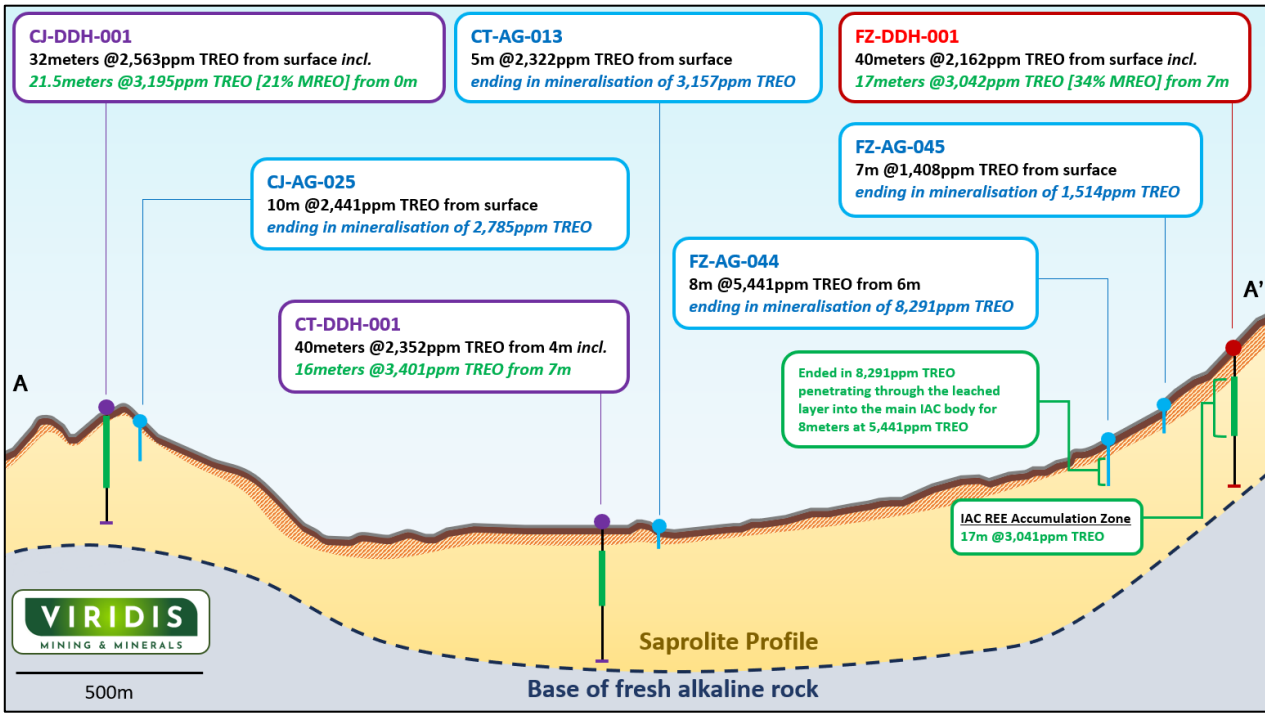
Figure 2: Geological interpretation of cross-section AA' going across the Northern Concessions as shown in Figure 1.
