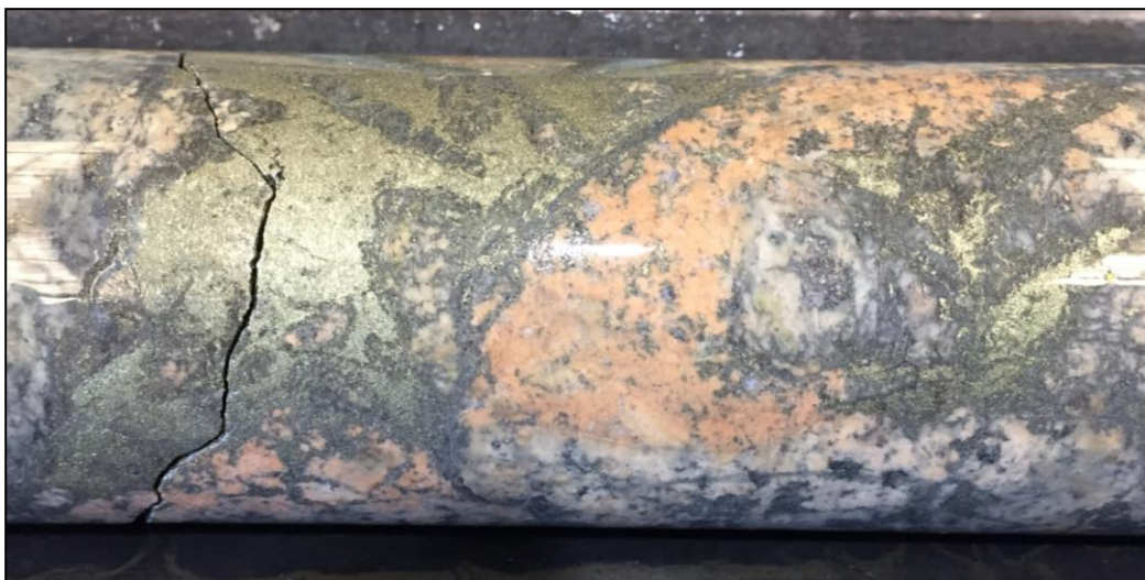
Figure 1. Breccia-hosted copper mineralisation west of the Corvette deposit, comprising 5.8 metres at 1.97% Cu & 179ppm Mo. This interval is one of the highest grade intersections ever drilled at the Myall Project (photograph from ~170 metres down hole in 23MYDD434, core diameter 45mm).
