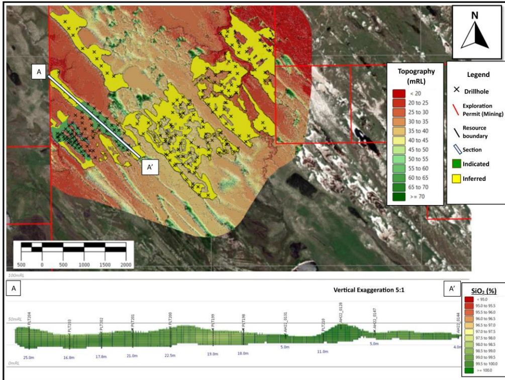
Long sections through the Western Resource Area block model. Section is exaggerated 5:1.
