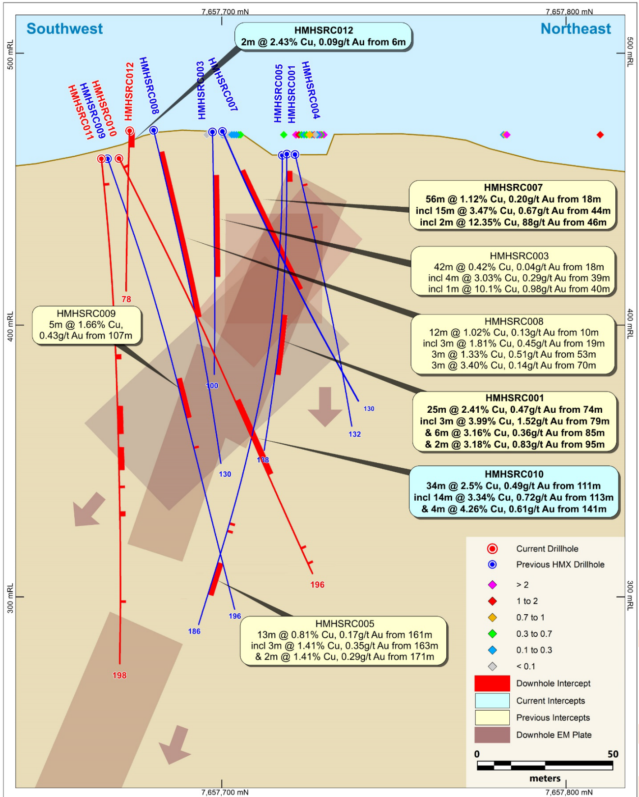
Figure 5. Hope South long section looking west showing the continuation of the conductive zone.
