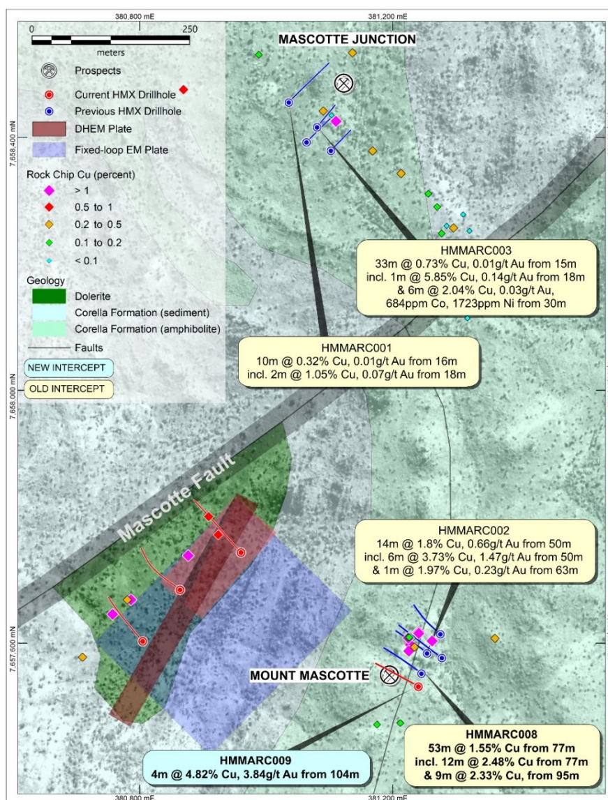
Figure 6. Mascotte region showing the location of drilling, significant intercepts, fixed loop and down-hole EM conductive plates.
