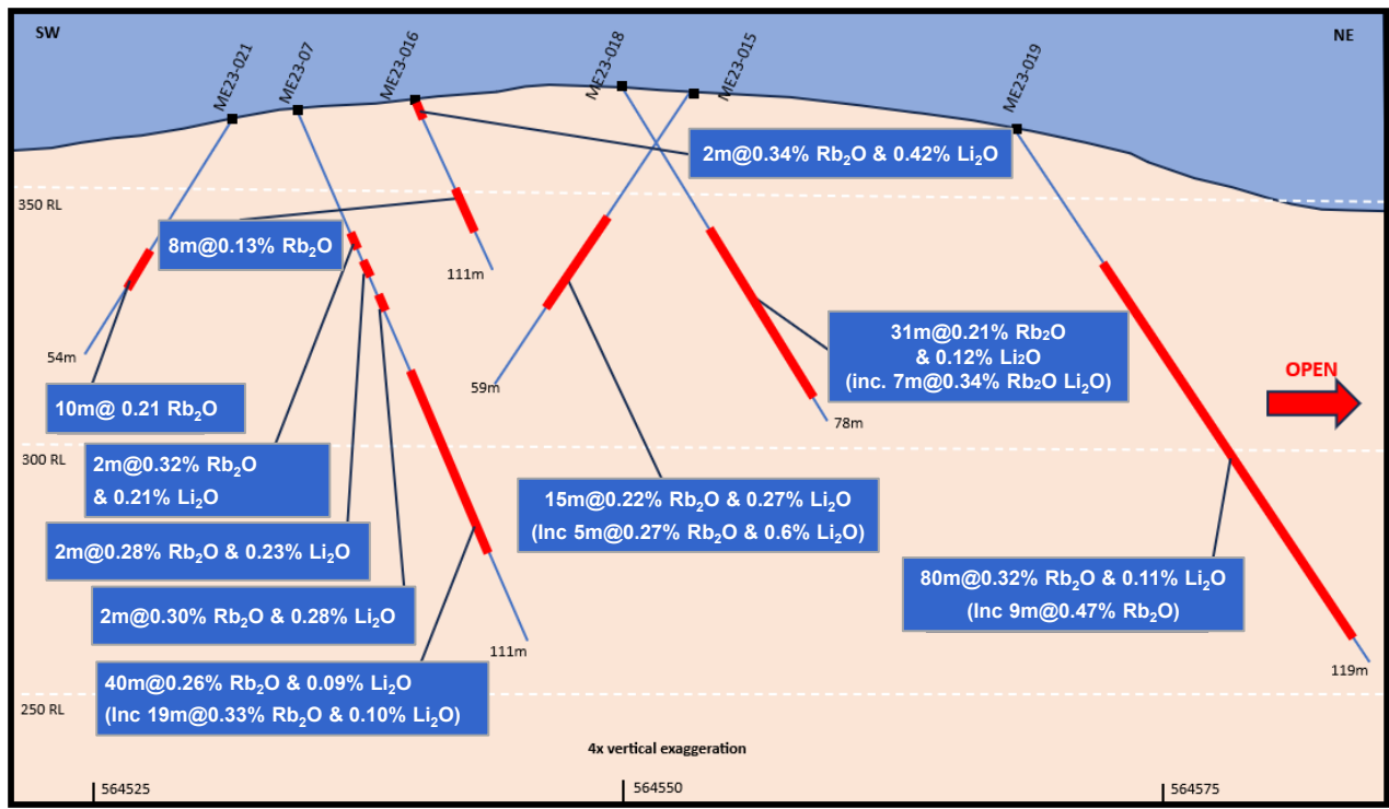
A schematic cross section looking northwest – Shows significant mineralised intersections in the northwest area of Mt Edon
