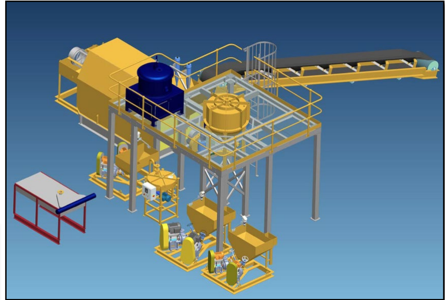
Gekko Mobile Gravity processing plant layout
