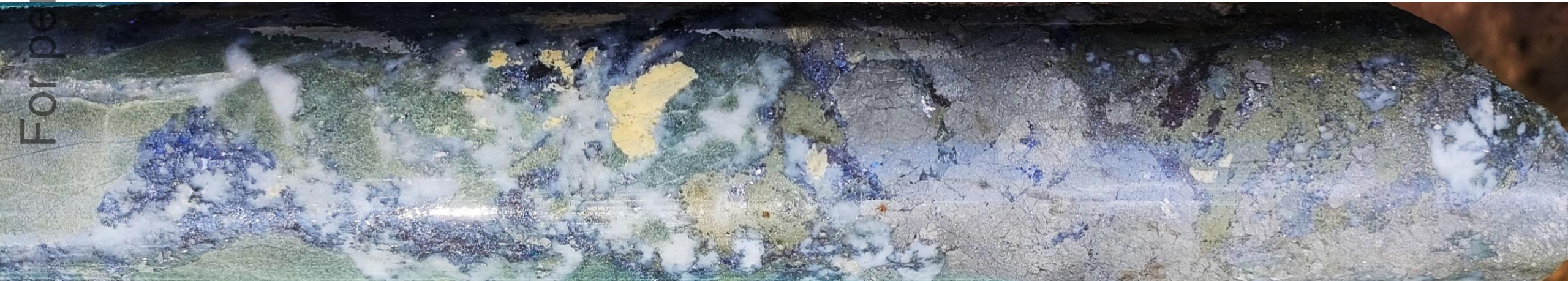
Trafalgar Prospect - Drill hole TFDD005 - Quartz-sulphide (pyrite-arsenopyrite-pyrrhotite-galena-sphalerite) vein at 120.3m (0.7m @ 152.5g/t Au)
