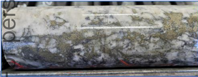
Quartz-sulphide vein with coarse pyrite-arsenopyrite-galenite in drill hole TFDD013 at 26m ( 0.5m @ 169.8g/t Au )
