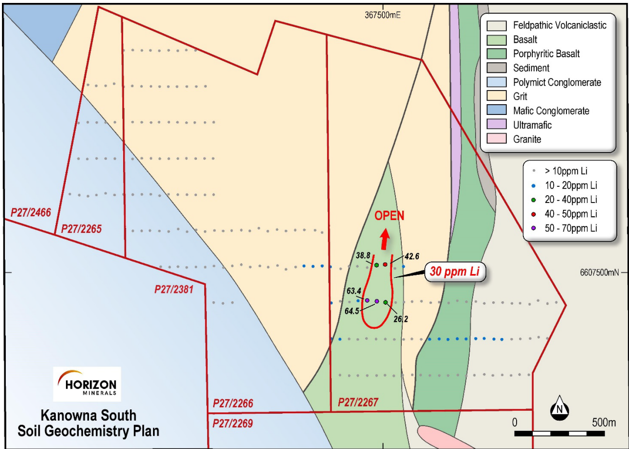
Figure 6: Kanowna South Li Geochemistry Plan
