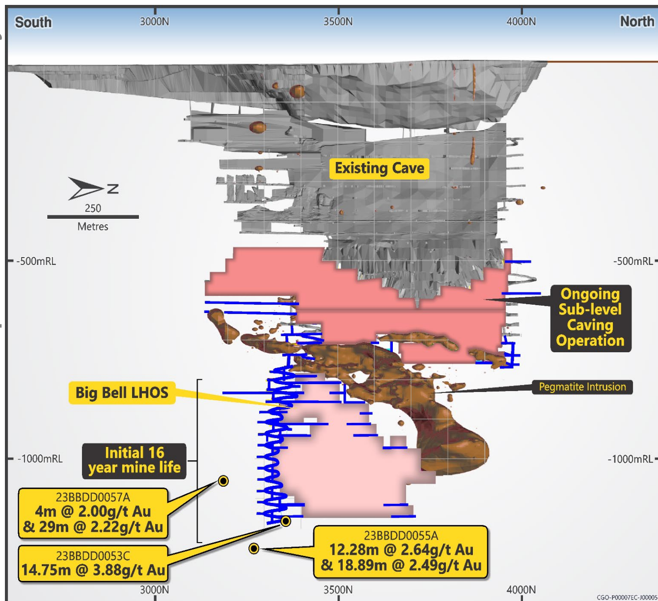
Figure 2 – Schematic of Big Bell Expansion Development plan
