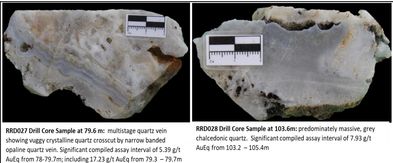
Figure 4: Photos of core specimens from Pertama vein drill holes RRD027 (above left) and RRD028 (above right) showing quartz textures and corresponding compiled assay intervals.
