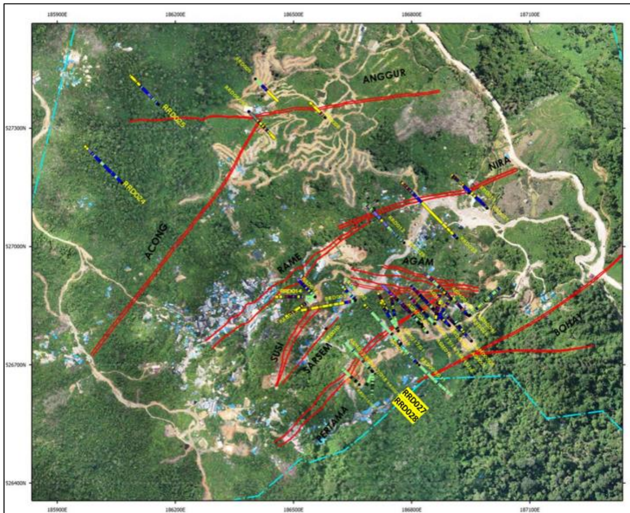
Figure 1: Plan map showing the surface extent of defined quartz vein zones in the southeastern part of the Rek Rinti prospect. The location of holes RRD027-RRD028 in the southwestern extension of the Pertama vein are indicated as are other holes completed as part of the Phase1 and 2 drill programs. Refer to Figure 2 for a schematic representation of the Rek Rinti quartz vein-breccia zones.
