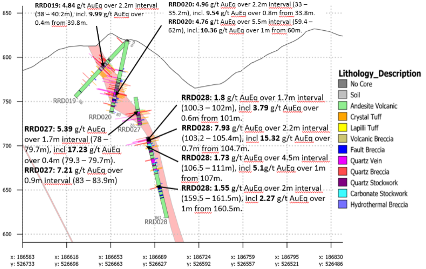
Figure 2: Interpreted cross section through the Pertama vein looking northeast. Compiled significant intersection for holes RRD027 and RRD028 are indicated. The Pertama vein has been the site of extensive historical artisanal mining which resulted in several intervals of no core recovered through the vein where drilled. Refer to Table 2. The Company will continue to test this zone at depth and along strike.
