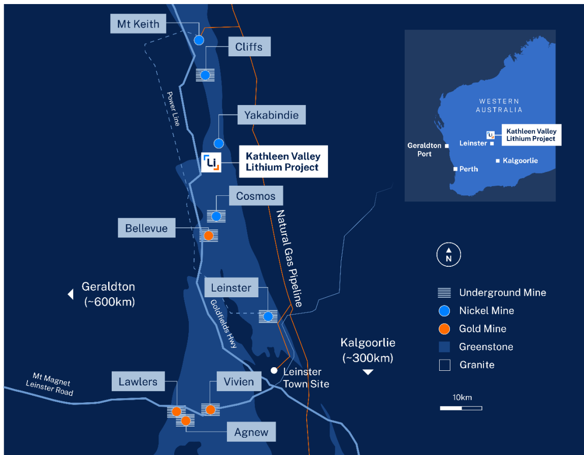
Figure 21: Kathleen Valley Lithium Project – Location and Geology Map
