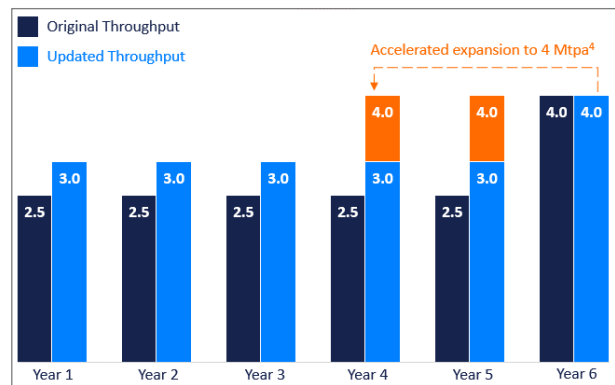
Figure 2: Kathleen Valley plant throughput capacity
