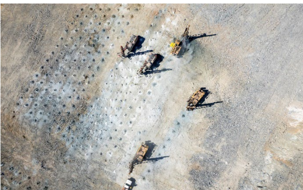
Figure 7: Blast preparation at Kathleen's Corner
