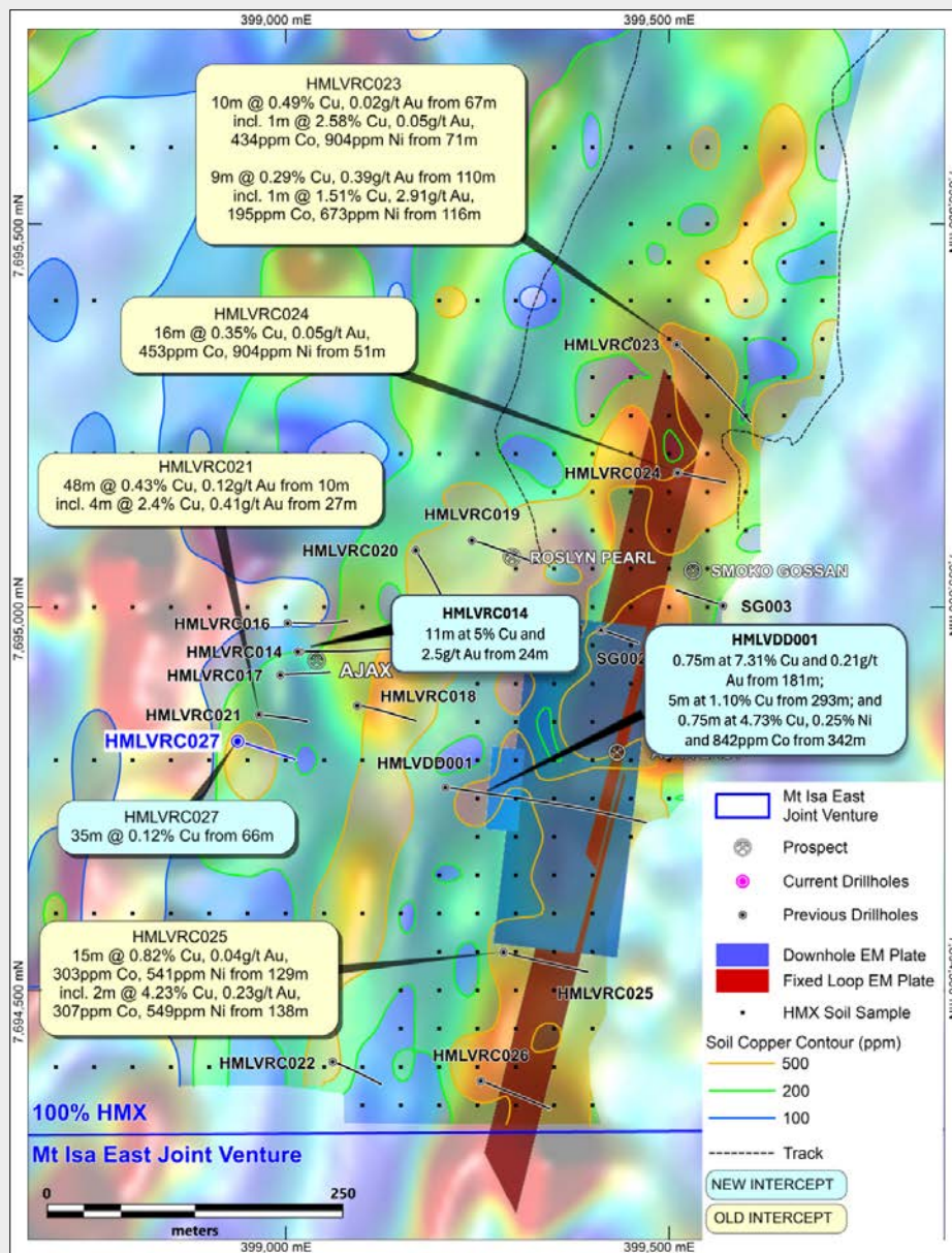
Ajax drilling highlights and underlying Electromagnetic Anomalies (See ASX Announcement 7 March 2023)
