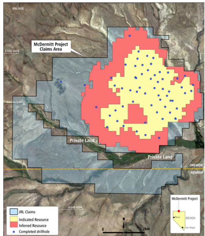
Plan view of the McDermitt Lithium Project with drill hole collars and 2023 Mineral Resource 4 (at 1523mRL)
