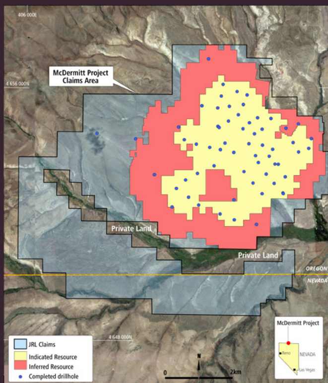
Plan view of the McDermitt Lithium Project with drill hole collars and 2023 Mineral Resource* (at 1523mRL)
