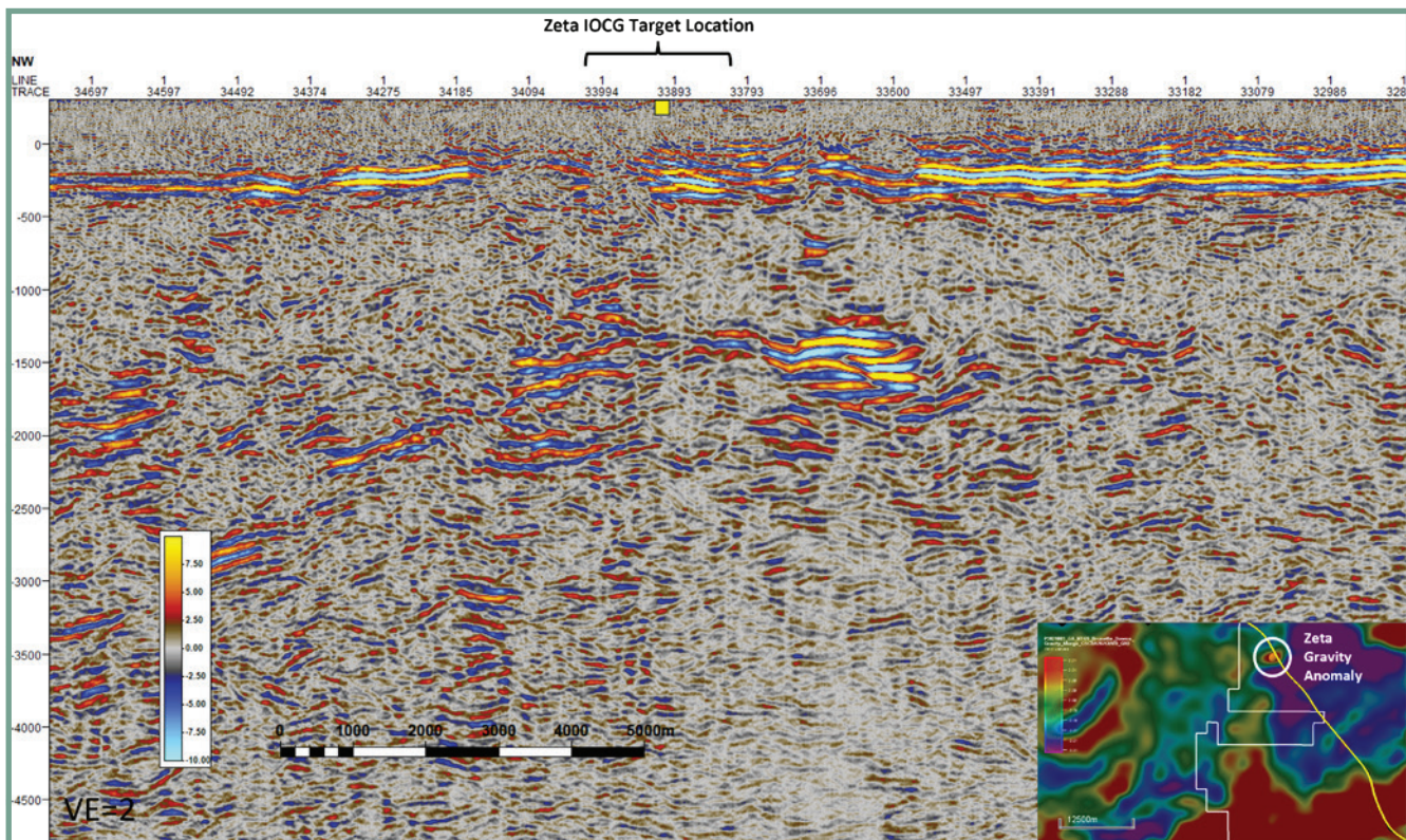
Figure 12 - Jessica Project - Zeta IOCG Target - Seismic cross section
