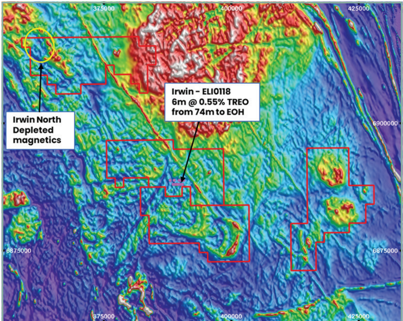
Figure 6 - RTP magnetic survey image highlighting the Irwin targets. Encounter tenements & historical aircore drillholes are shown
