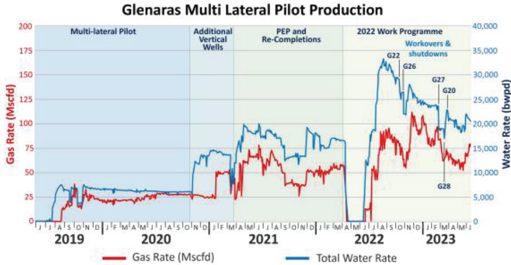
Glenaras Pilot water and gas production history
